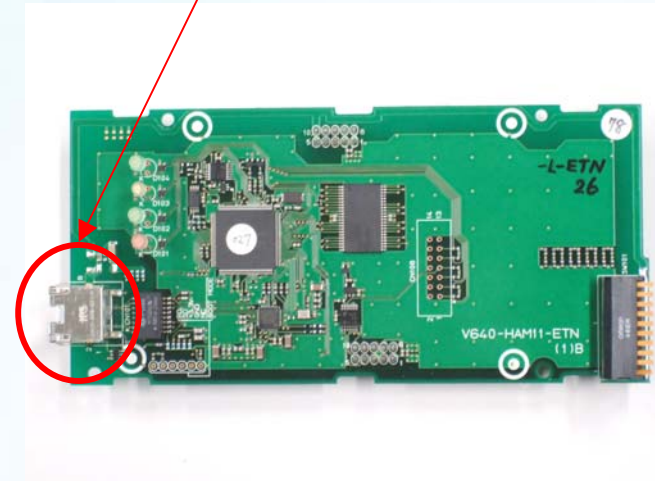
Inside of V640-HAM11-ETN
