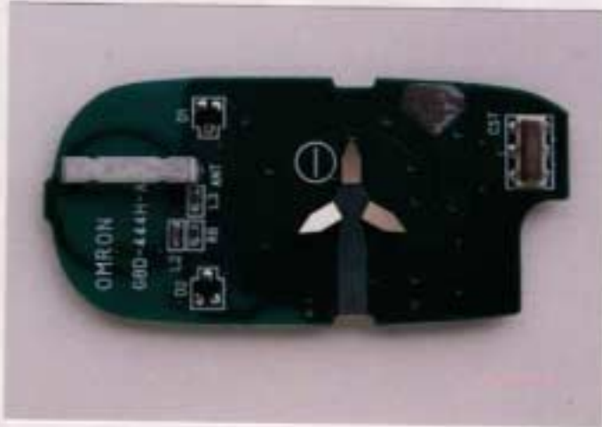
Figure 8.4 PCB assy (back view)
