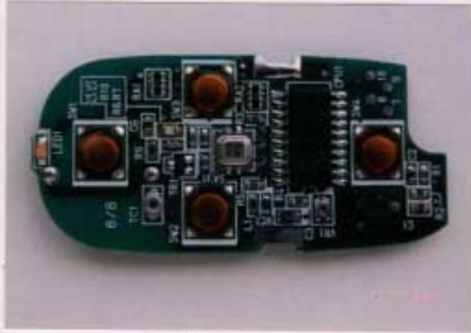
Figure 8.3 PCB assy (front view)
