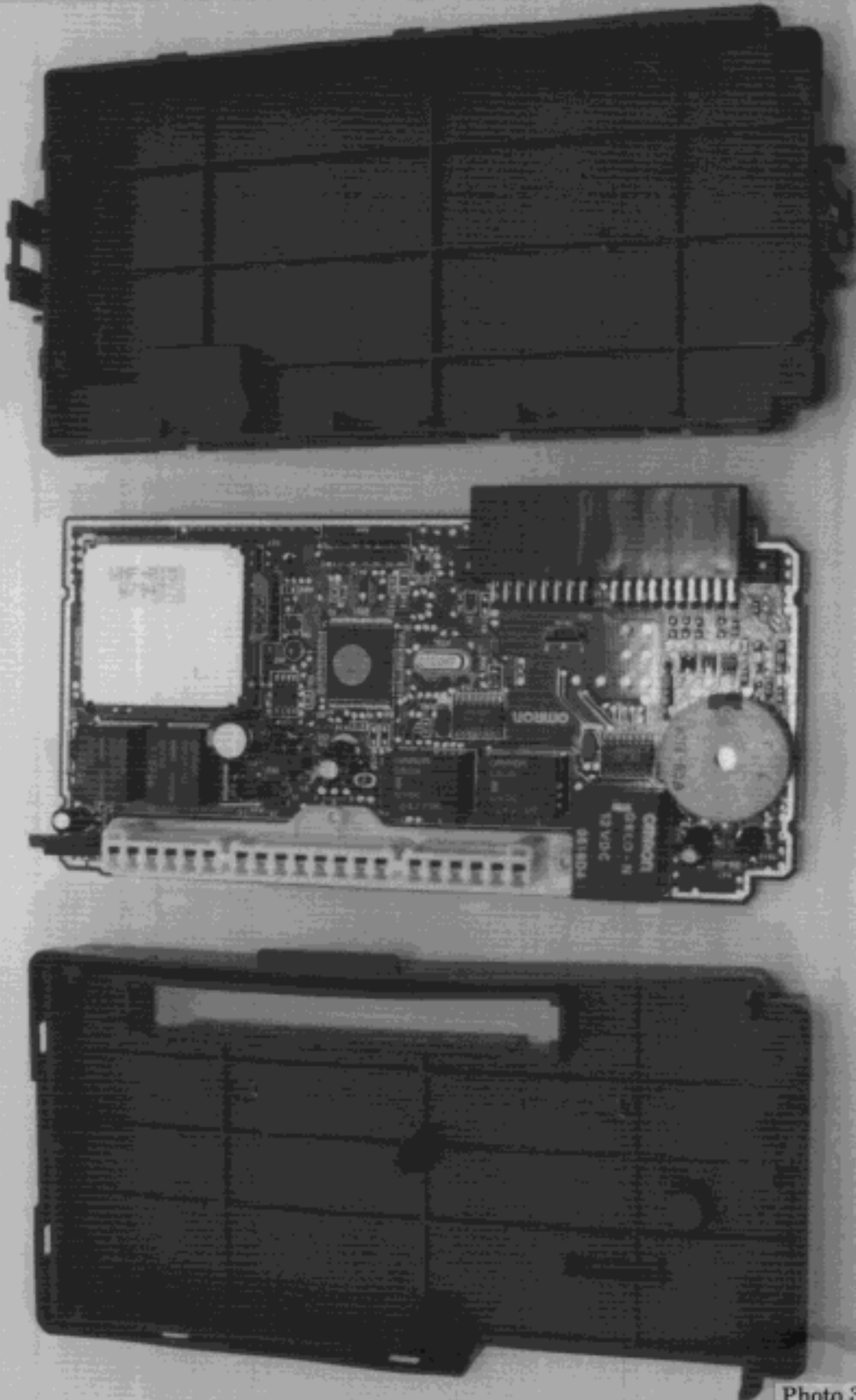
Photo 3 Cover Taken Off GSC-253M OMRON Corporation
