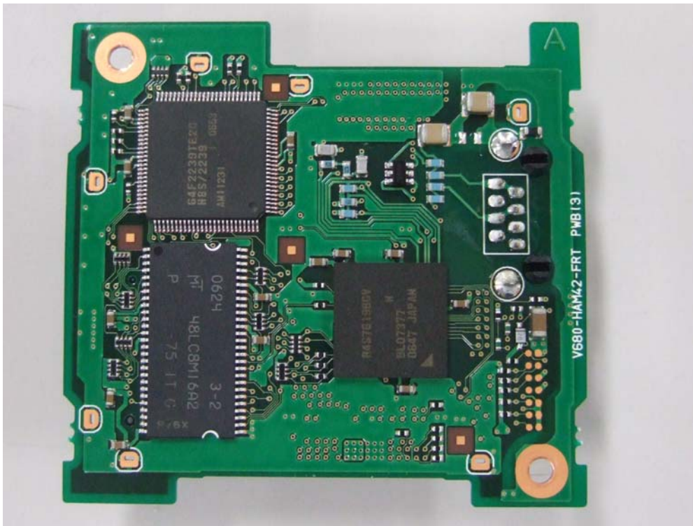
PWB (3) Side B
