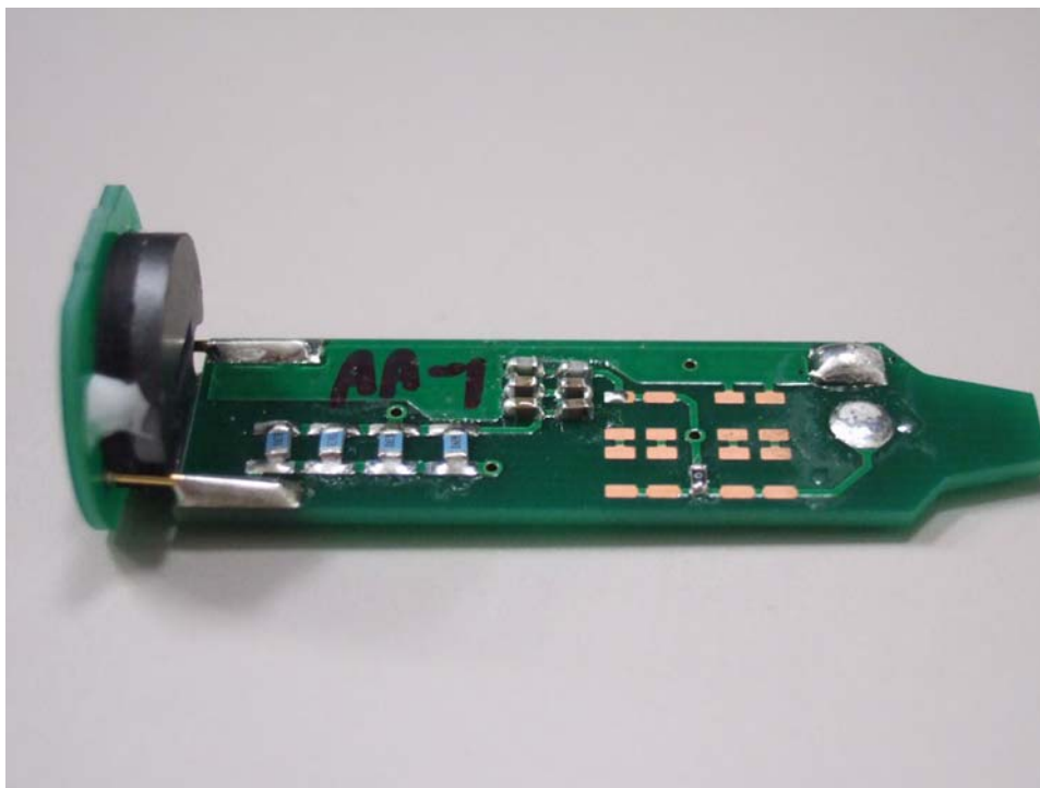
Composition Side D of Antenna (V680-HS52)
