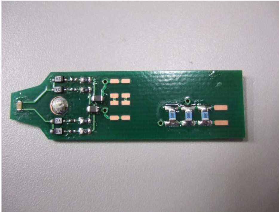
PWB (2) Side A of Antenna (V680-HS52)
