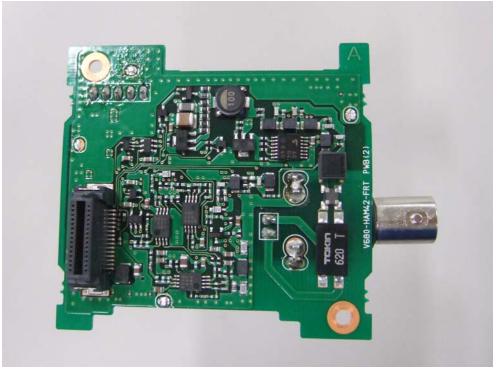
PWB (2) Side B without shield
