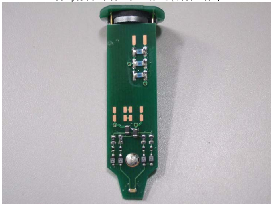
Composition Side B of Antenna (V680-HS52)
