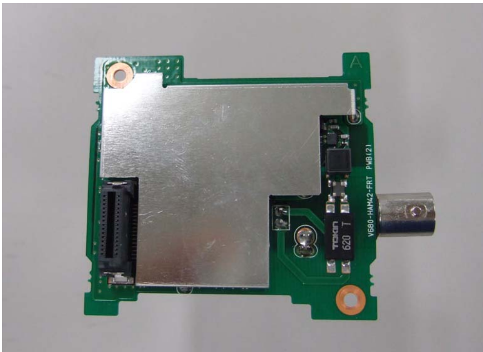
PWB (2) Side B with shield
