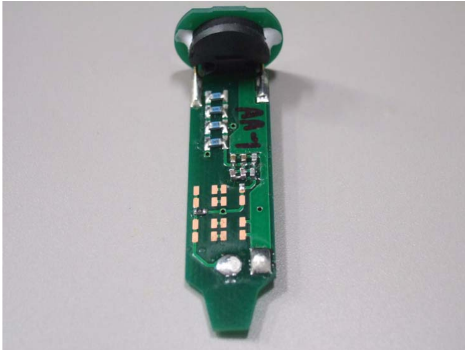
Composition Side A of Antenna (V680-HS52)
