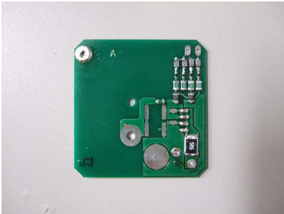
PWB (2) Side A of Antenna (V680-HS63)
