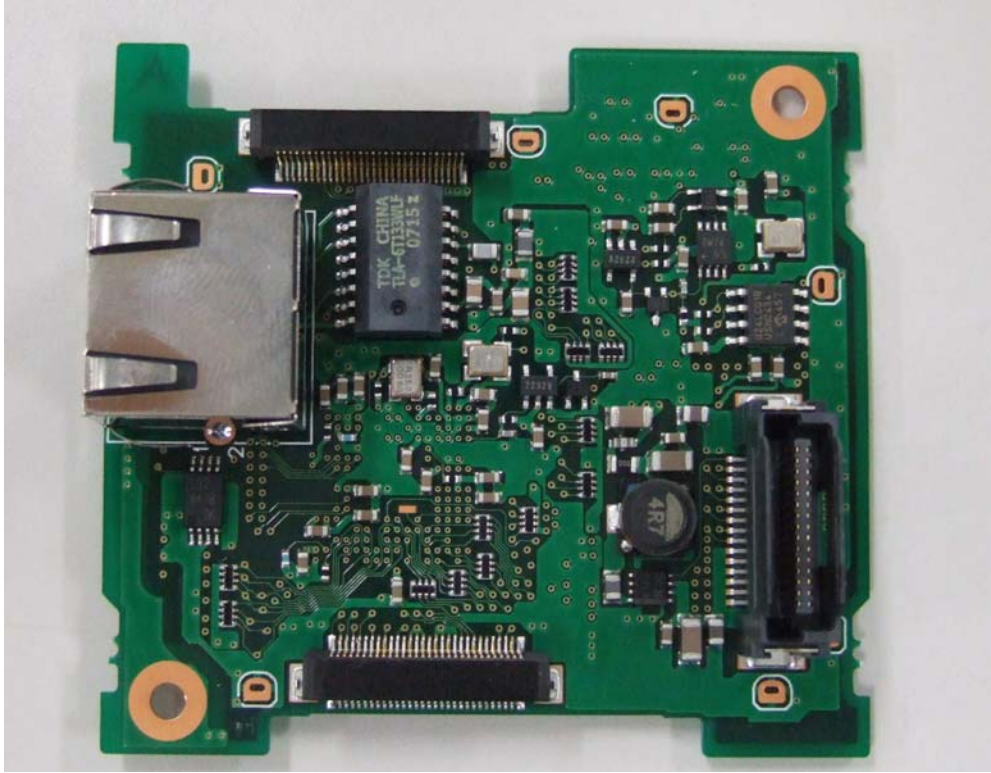
PWB (3) Side A
