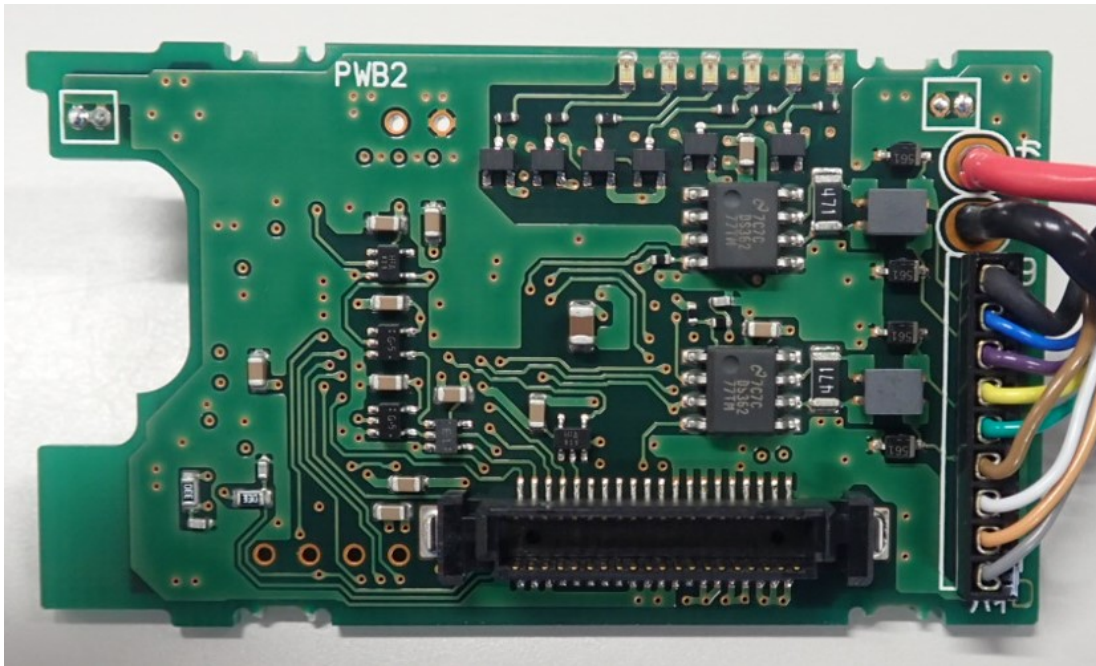
One side of the Printed-Circuit Board No.2
