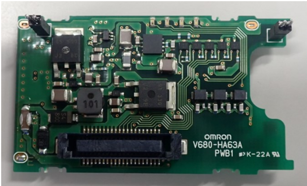
One side of the Printed-Circuit Board No.1
