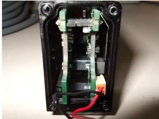
PWB(1) and PWB (2) in Case (V680-HA63)
