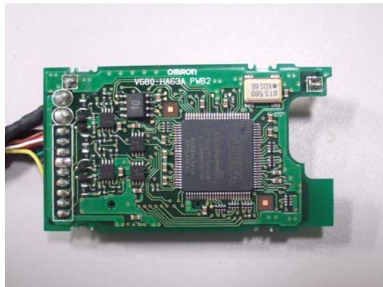
PWB (2) Side B (V680-HA63)
