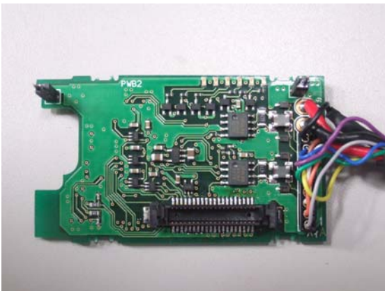
PWB (2) Side A (V680-HA63)
