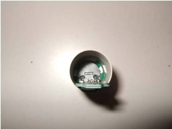
PWB(1) and PWB (2) in Case (V680-HS52)
