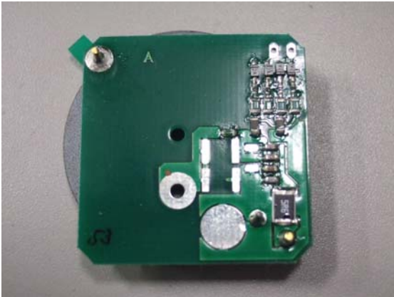
Composition Side B (V680-HS63)
