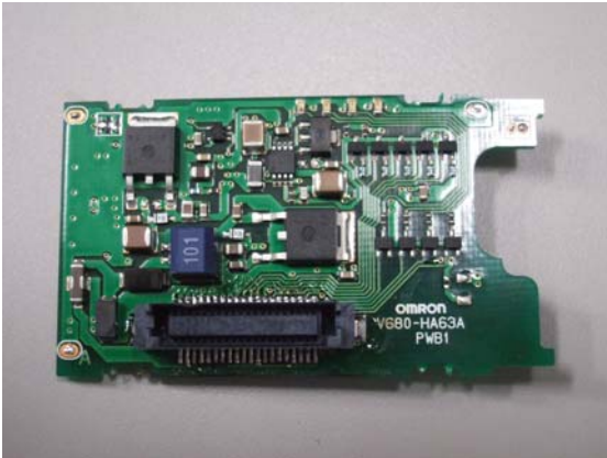
PWB (1) Side A (V680-HA63)
