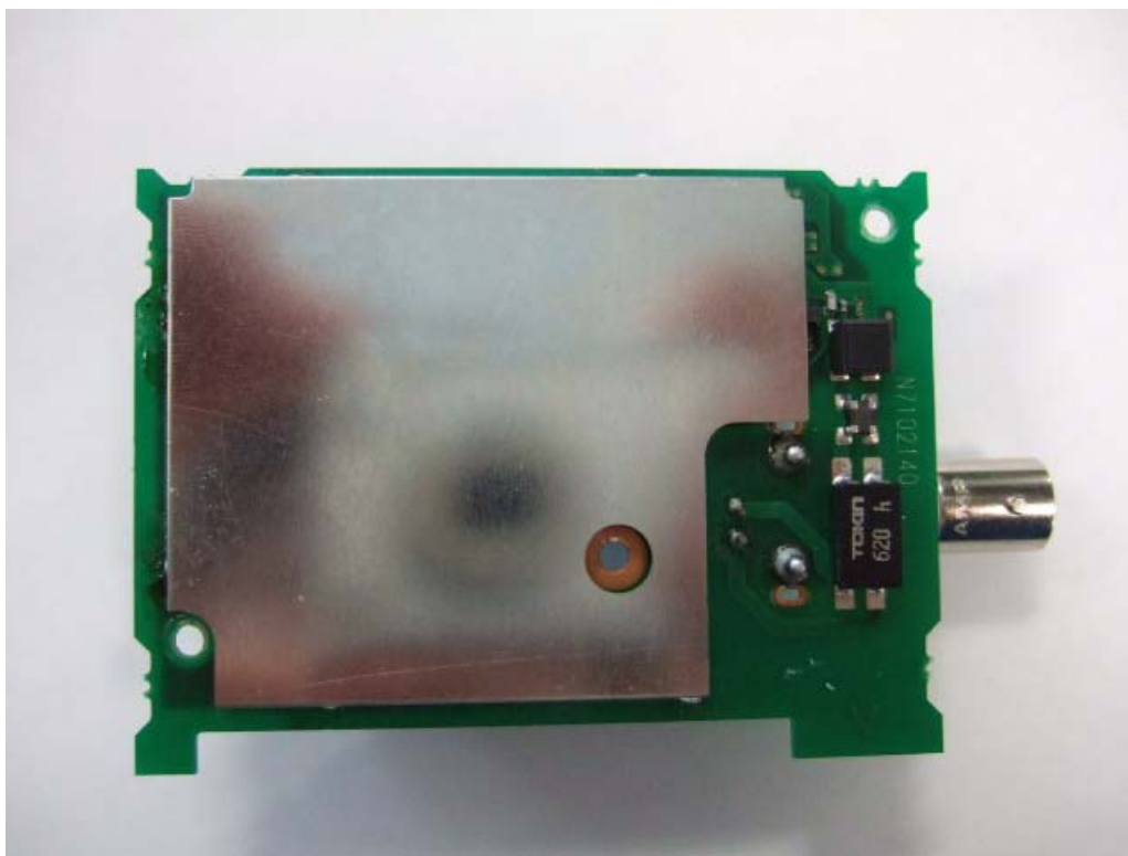
Top of PWB(2) with shield
