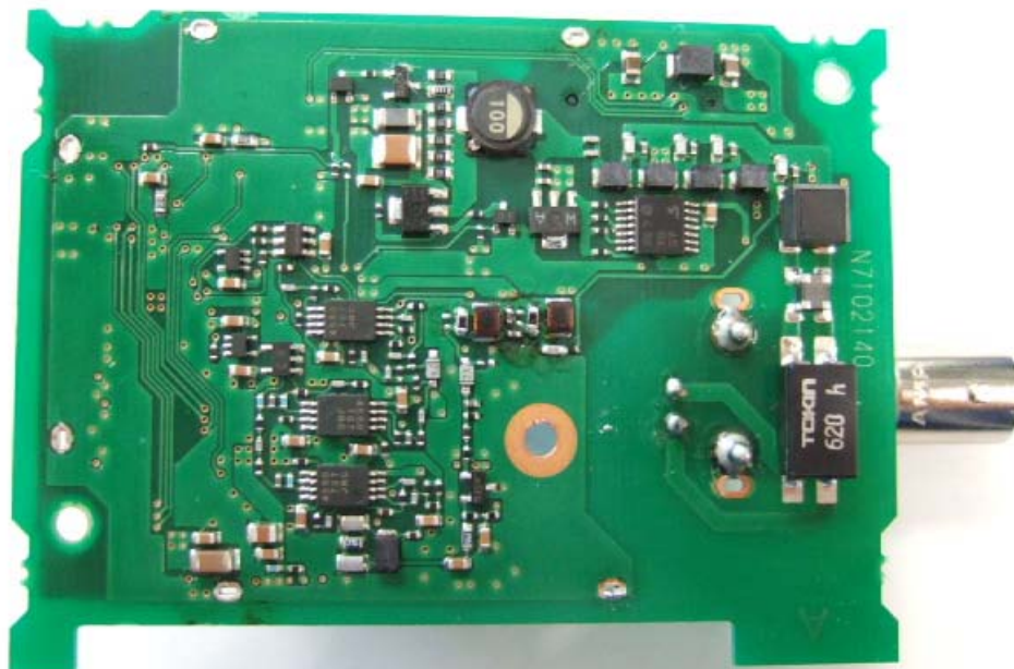
Top of PWB(2) without shield
