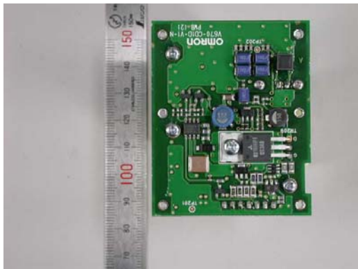
Side A (Transmission circuit)
