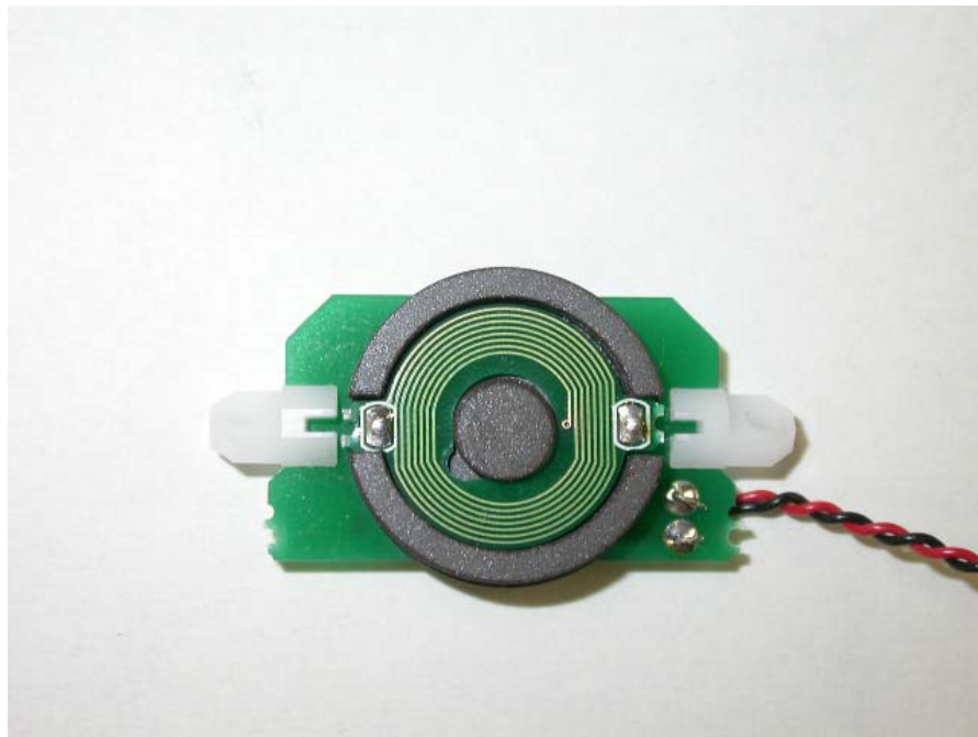
PWB (3) – Side B
