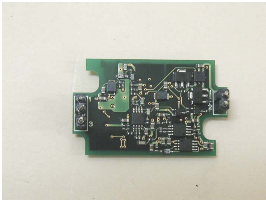
PWB (2) – Side B
