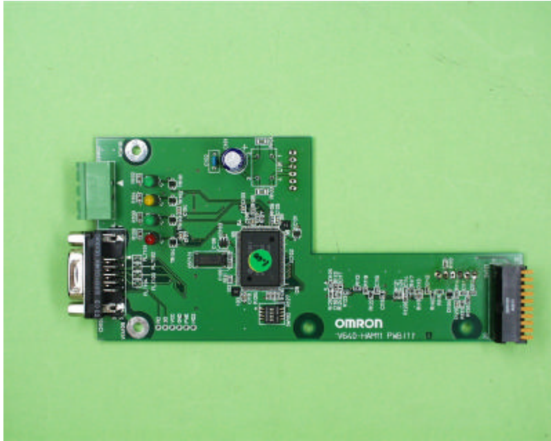
Upper Circuit Board (Front)
