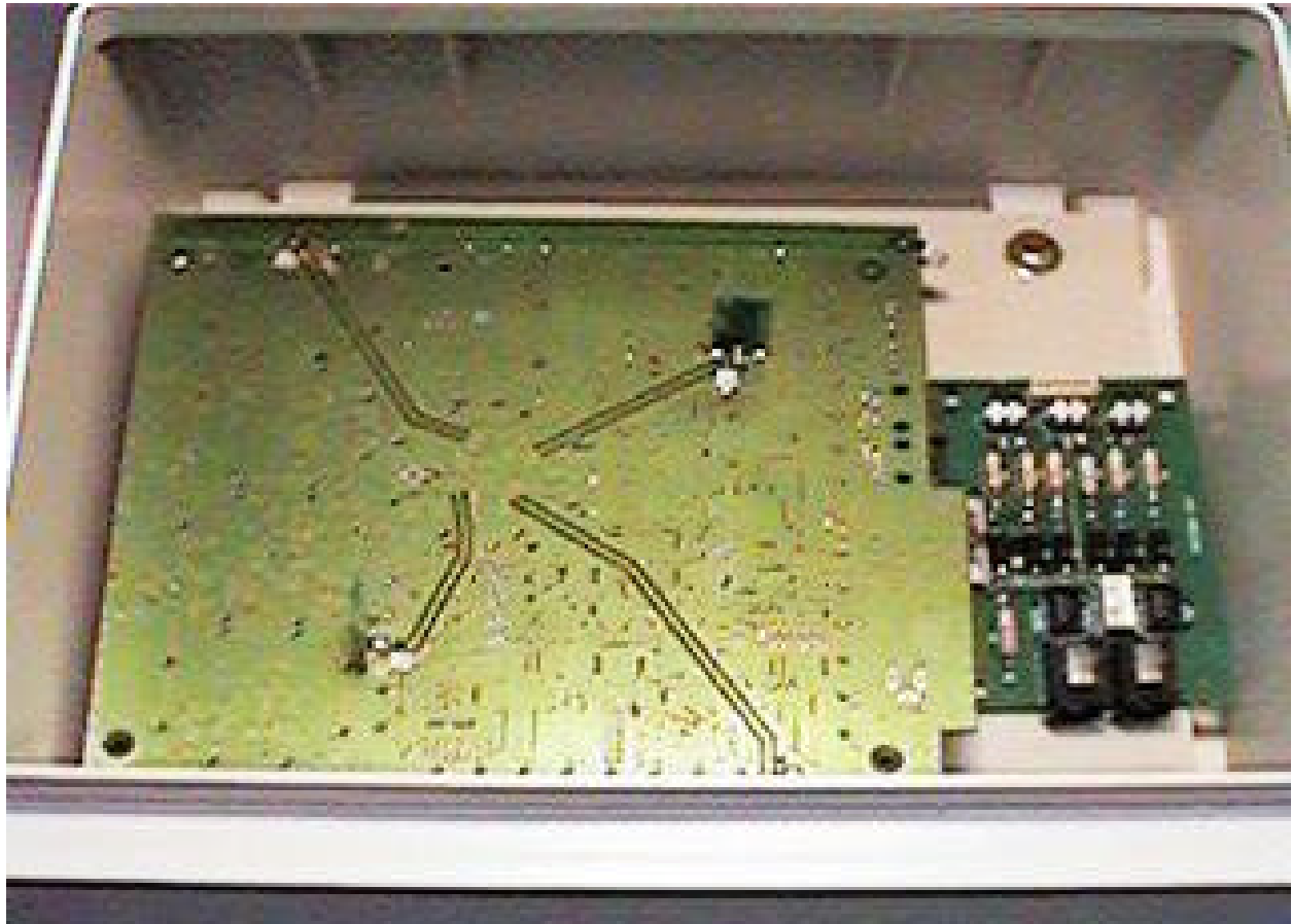
Inside View of the Outdoor Unit
