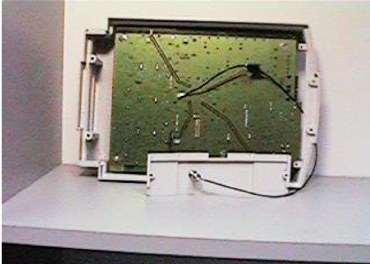
Inside View of the Five Antenna Unit (External Antenna)
