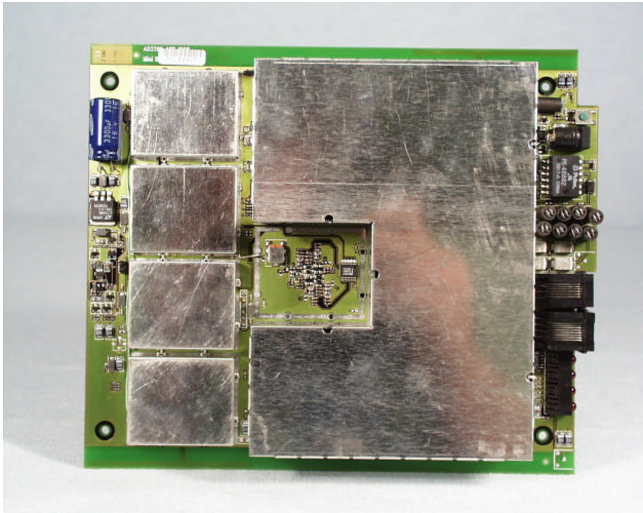
Component Side of the Mini Base (with RF covers installed)
