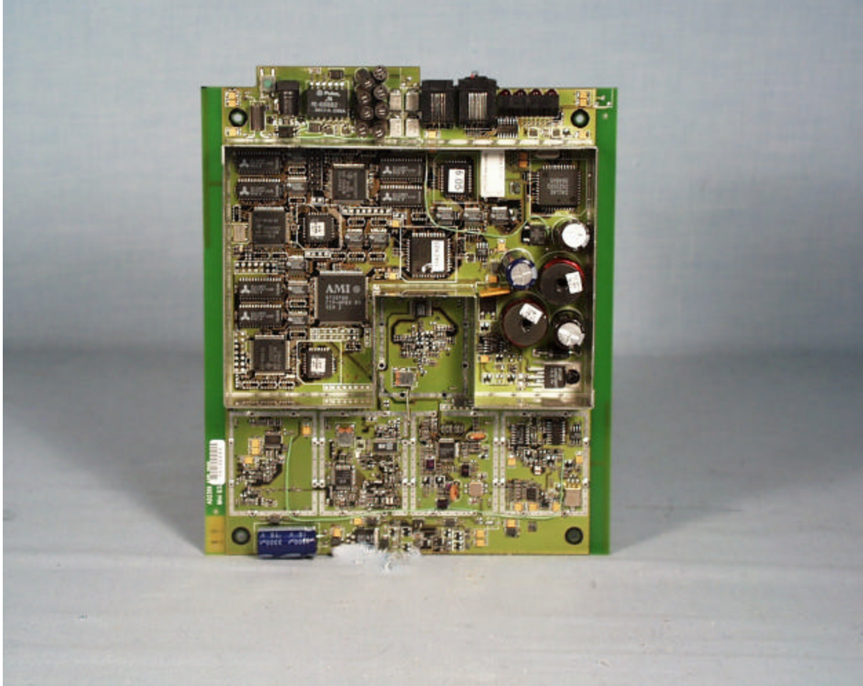
Component Side of the Mini Base (with RF covers removed)
