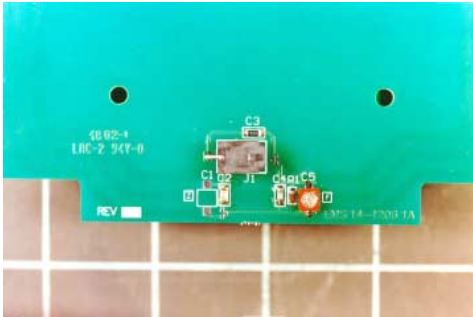
Antenna Connector Close-up
