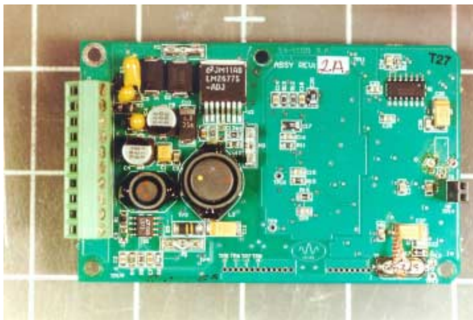
Top Main PCB with cans removed
