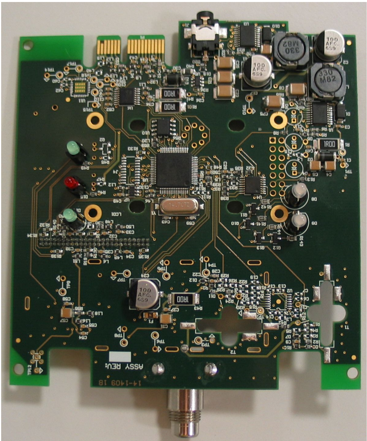
Top Side GEL-3232 PCB ASSY Main HF-CNTL-PBS-02:
