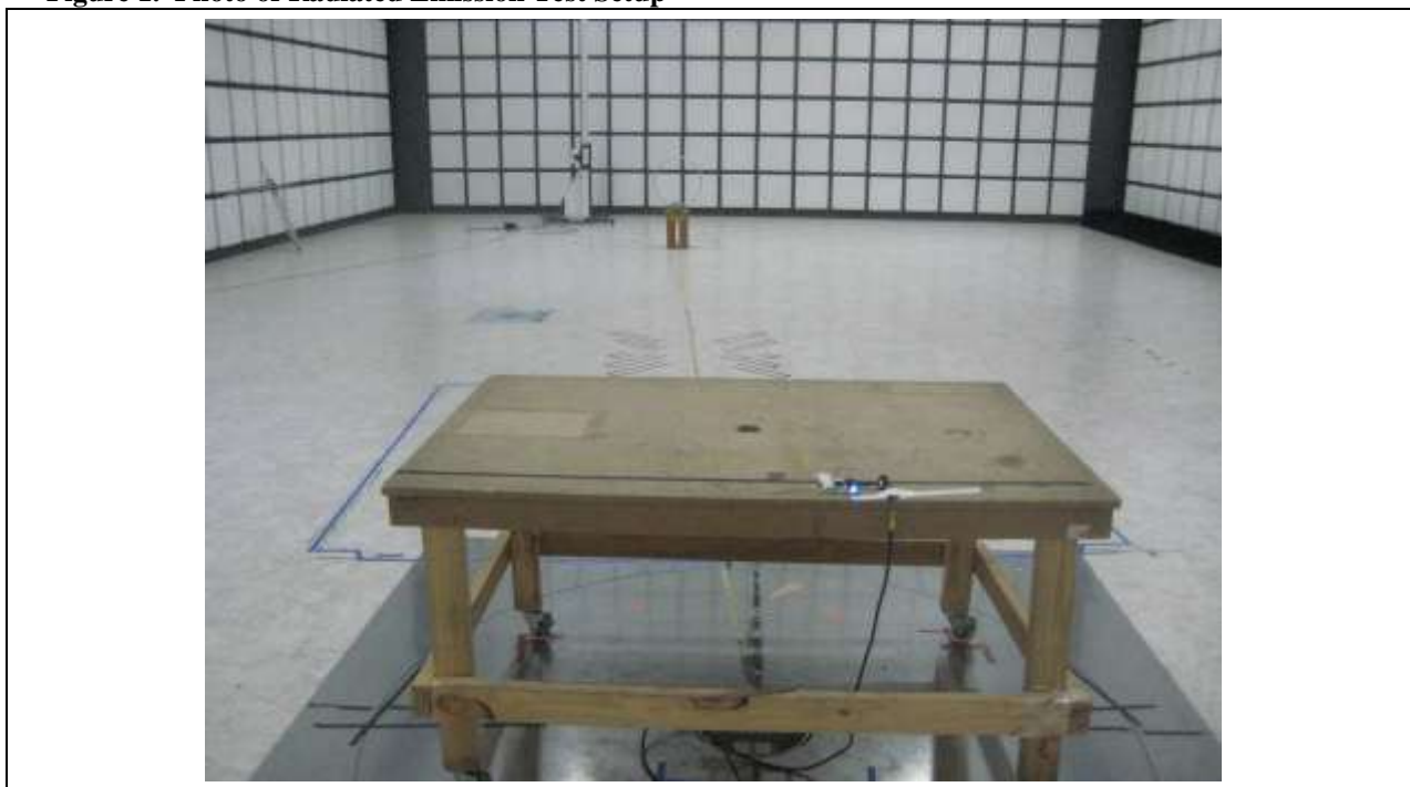
Figure 1. Photo of Radiated Emission Test Setup
