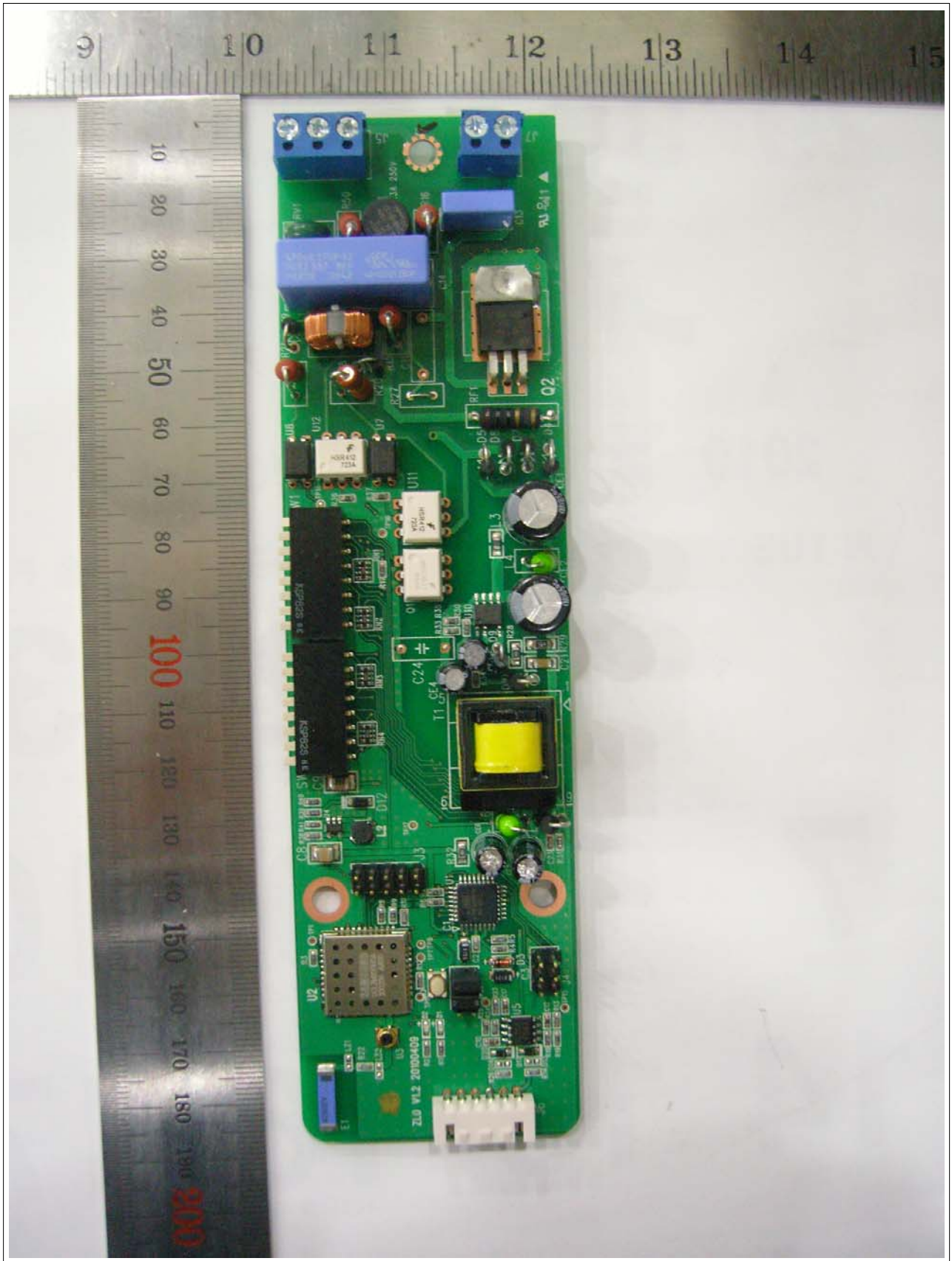
View of Main PCB(Top) - Shield Cover mounting state
