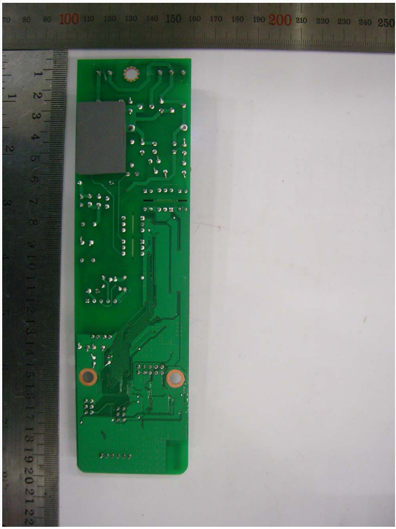
View of Main PCB(Bottom) - Gab pad mounting state
