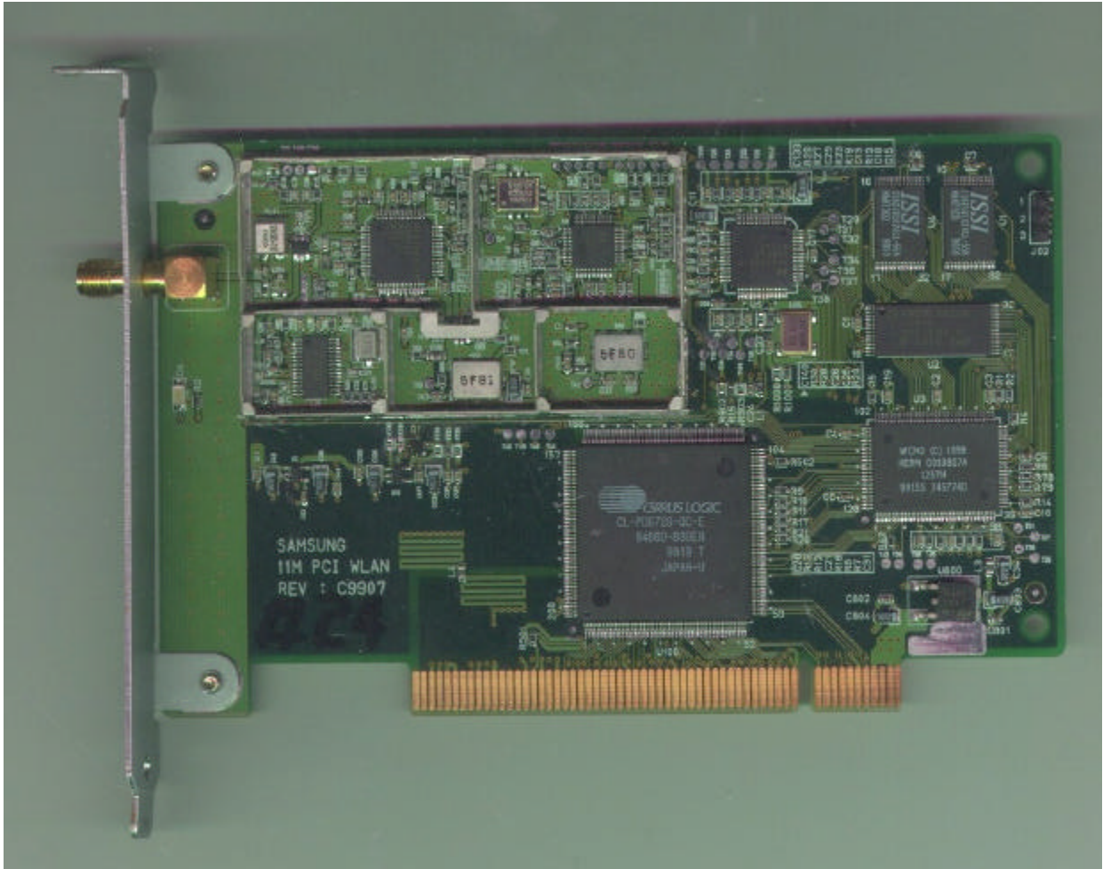
Figure 3: PCI Board Component Side
