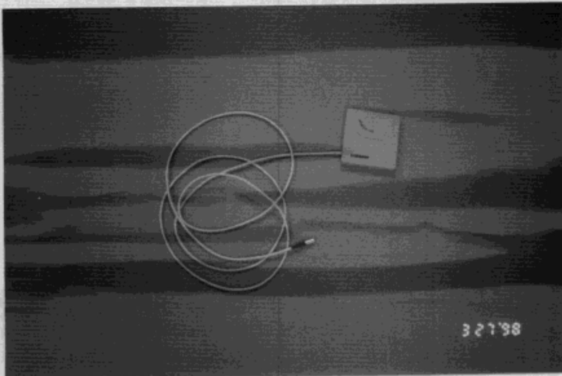
Figure 9.2 Antenna Assembled
