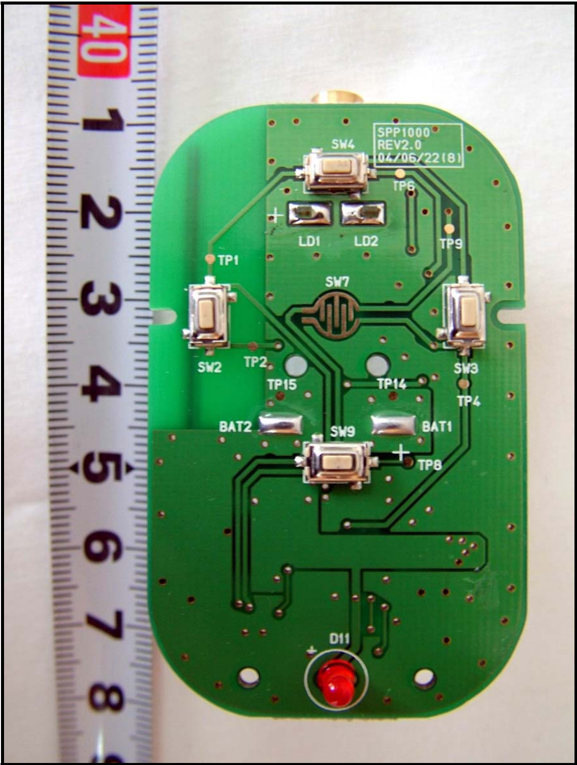
Front View of PCB
