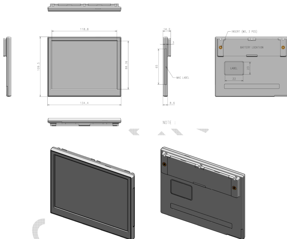
Figure 2 Mechanical Dimension
