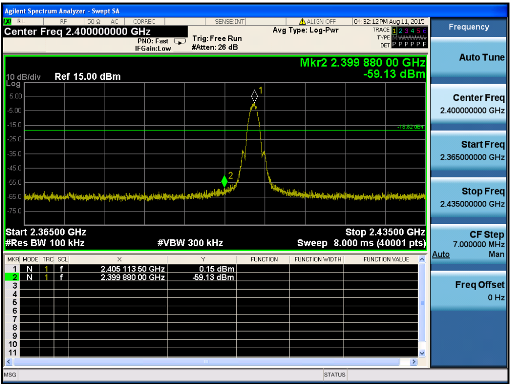
Low Band-edge
