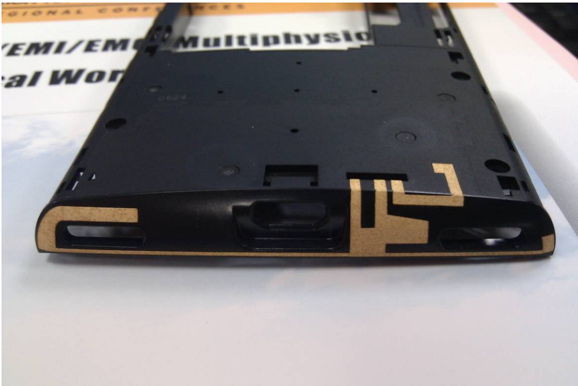
Internal View of EUT – 9 (WWAN antenna)
