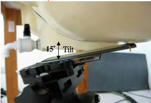
Fig.10 Left Head Section / Ear-Tilt Position(15°)_ Slider on
