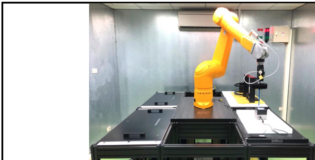
Fig-3.2 SPEAG DASY6 System
