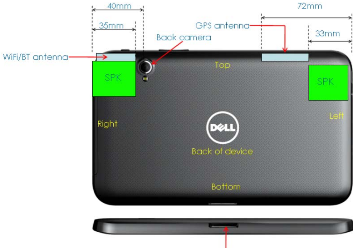
Fig.9 Antenna position of EUT
