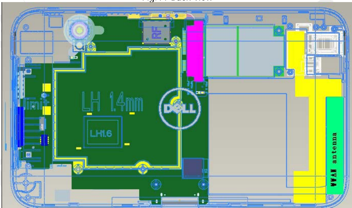
Fig.12 Proximity sensor portion in Yellow (from back view)
