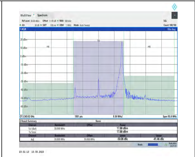
1-N48-PC3-30-30-L-CP-QPSK-Edge_1RB_Left-1@7 7-Ant1-1--PASS
