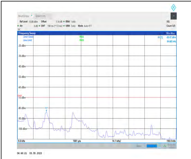
1-N48-PC3-30-40-M-1-DFT-PI2BPSK-Inner_1RB_Le ft-1@1-0.009-0.15-Ant1-0.01--112.00--70-PASS
