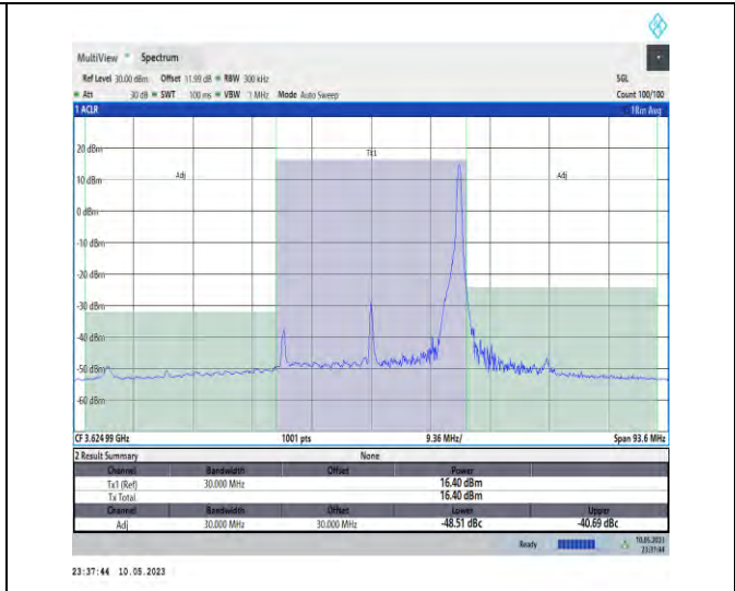
1-N48-PC3-30-30-M-CP-QPSK-Edge_1RB_Left-1@7 7-Ant1-1--PASS
