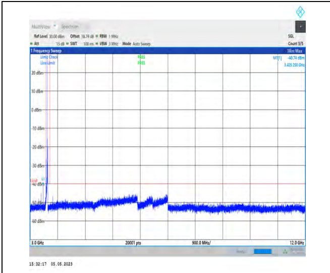
1-N48-PC3-30-40-L-1-DFT-PI2BPSK-Inner_1RB_Lef t-1@1-3000-12000-Ant1-3496.80--40.74--40-PASS
