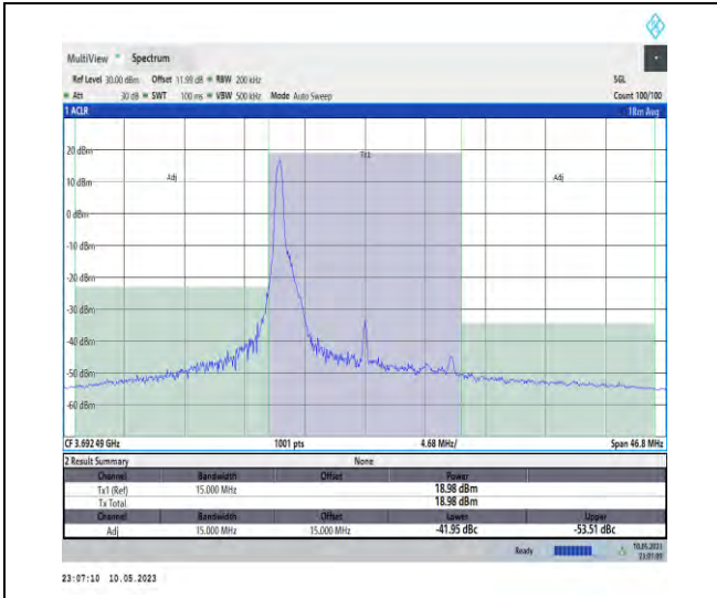
1-N48-PC3-30-15-H-DFT-PI2BPSK-Edge_1RB_Left -1@0-Ant1-1--PASS
