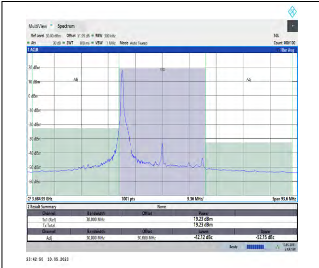
1-N48-PC3-30-30-H-DFT-PI2BPSK-Edge_1RB_Left-1@0-Ant1-1--PASS
