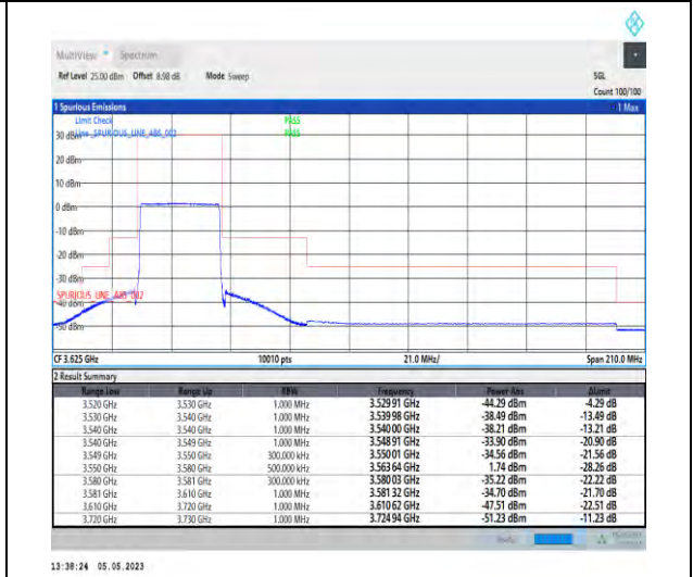
1-N48-PC3-30-30-L-6-CP-QPSK-Outer_Full-78@0-Ant1-1--PASS-see graph
