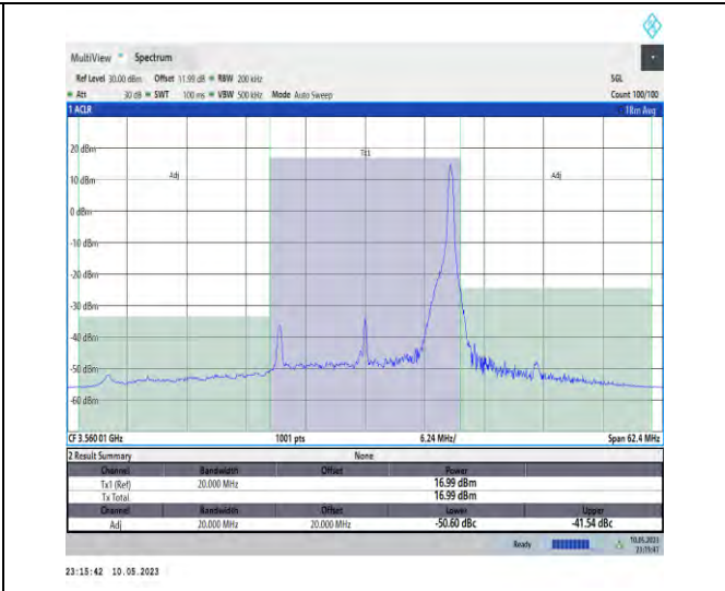
1-N48-PC3-30-20-L-CP-QPSK-Edge_1RB_Left-1@5 0-Ant1-1--PASS
