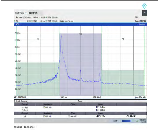
1-N48-PC3-30-20-L-DFT-PI2BPSK-Edge_1RB_Left-1@0-Ant1-1--PASS
