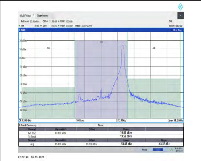
1-N48-PC3-30-10-L-DFT-PI2BPSK-Edge_1RB_Left-1@23-Ant1-1--PASS
