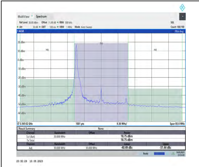
1-N48-PC3-30-30-L-DFT-PI2BPSK-Edge_1RB_Left -1@0-Ant1-1--PASS
