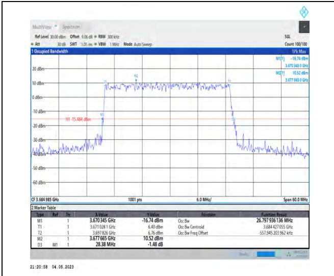
1-N48-PC3-30-30-H-2-DFT-PI2BPSK-Outer_Full-75 @0-Ant1-26.798-28.380-<30-PASS
