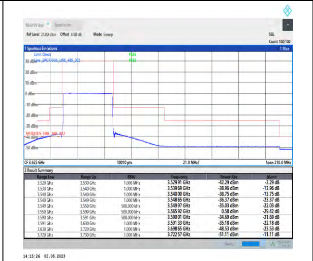
1-N48-PC3-30-40-L-6-CP-QPSK-Outer_Full-106@0-Ant1-1--PASS-see graph
