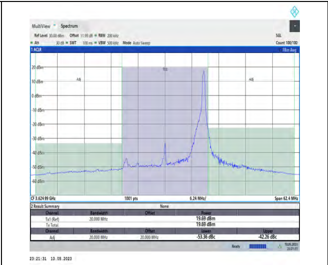
1-N48-PC3-30-20-M-DFT-PI2BPSK-Edge_1RB_Left-1@50-Ant1-1--PASS
