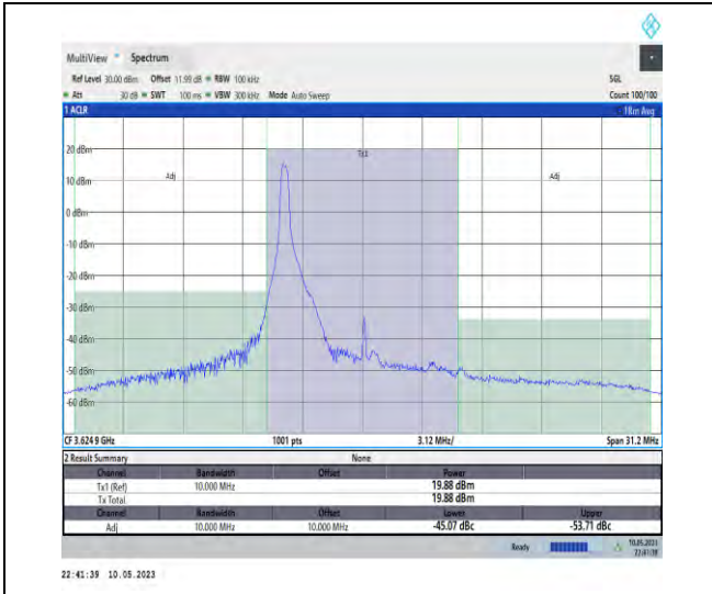
1-N48-PC3-30-10-M-DFT-PI2BPSK-Edge_1RB_Left-1@0-Ant1-1--PASS
