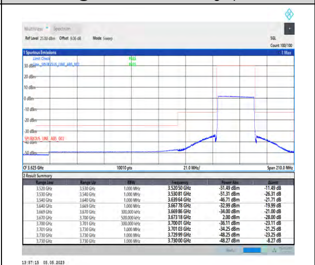
1-N48-PC3-30-30-H-6-CP-QPSK-Outer_Full-78@0-Ant1-1--PASS-see graph
