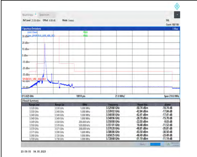
1-N48-PC3-30-20-L-4-CP-QPSK-Edge_1RB_Left-1@0-Ant1-1--PASS-see graph
