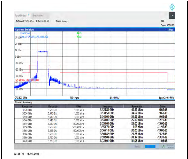
1-N48-PC3-30-15-L-3-DFT-PI2BPSK-Outer_Full-36@0-Ant1-1--PASS-see graph
