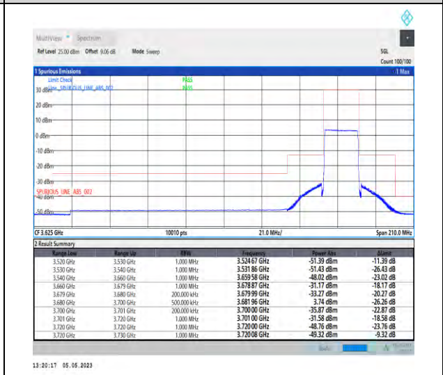
1-N48-PC3-30-20-H-6-CP-QPSK-Outer_Full-51@0-Ant1-1--PASS-see graph
