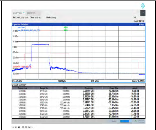
1-N48-PC3-30-30-L-3-DFT-PI2BPSK-Outer_Full-75@0-Ant1-1--PASS-see graph
