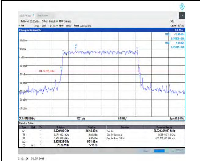
1-N48-PC3-30-30-H-4-DFT-64QAM-Outer_Full-75@ 0-Ant1-26.729-28.260-<30-PASS
