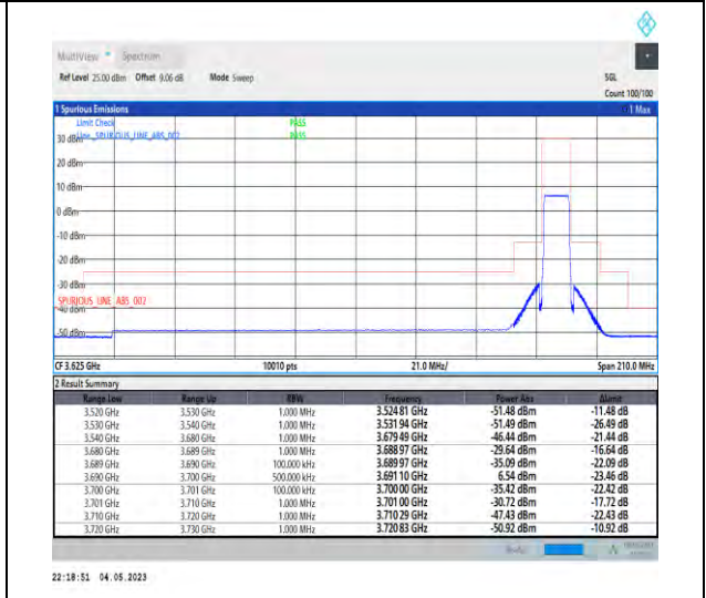
1-N48-PC3-30-10-H-6-CP-QPSK-Outer_Full-24@0-Ant1-1--PASS-see graph
