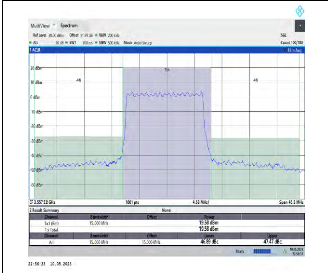
1-N48-PC3-30-15-L-DFT-PI2BPSK-Outer_Full-36@0-Ant1-1--PASS
