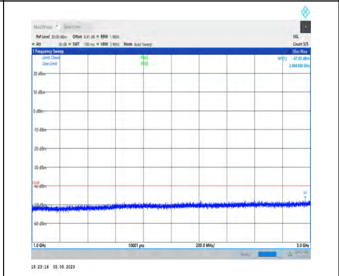
1-N48-PC3-30-40-H-1-DFT-PI2BPSK-Inner_1RB_Le ft-1@1-1000-3000-Ant1-2677.60--47.03--40-PASS
