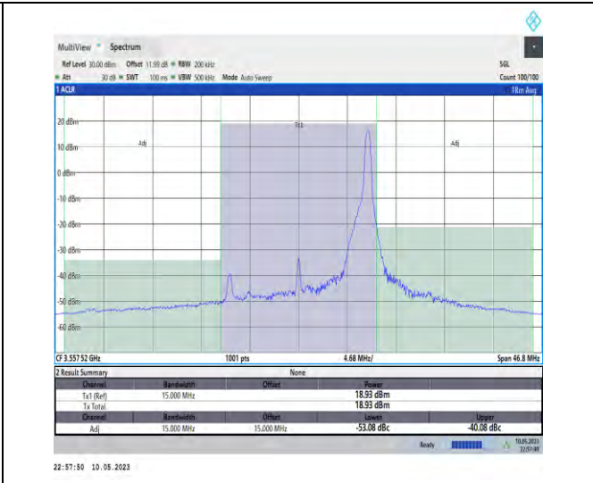
1-N48-PC3-30-15-L-DFT-PI2BPSK-Edge_1RB_Left-1@37-Ant1-1--PASS
