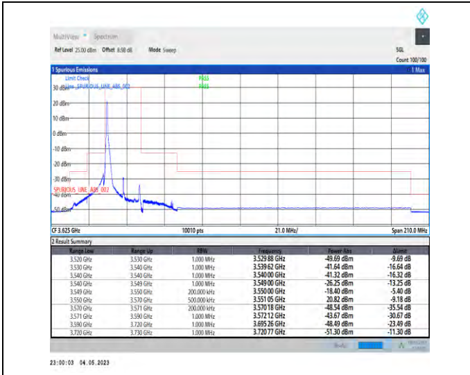
1-N48-PC3-30-20-L-1-DFT-PI2BPSK-Edge_1RB_Left-1@0-Ant1-1--PASS-see graph
