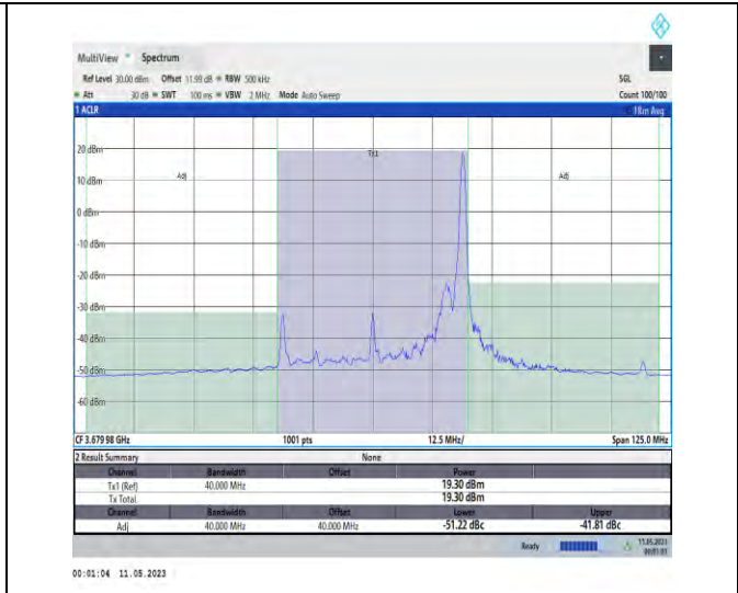
1-N48-PC3-30-40-H-DFT-PI2BPSK-Edge_1RB_Left-1@105-Ant1-1--PASS
