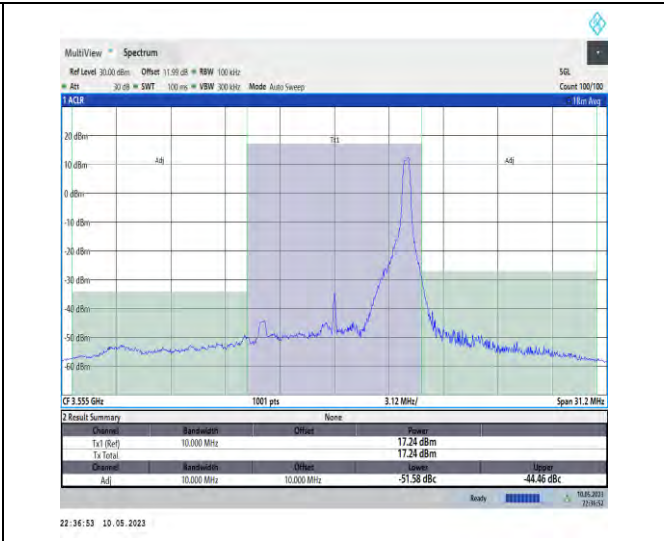
1-N48-PC3-30-10-L-CP-QPSK-Edge_1RB_Left-1@2 3-Ant1-1--PASS
