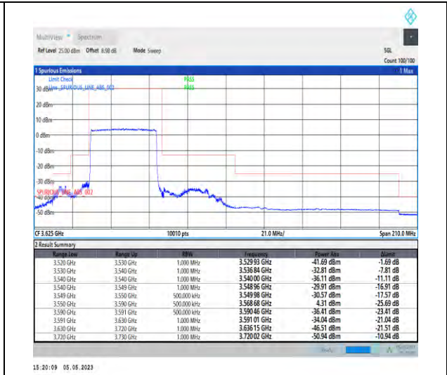
1-N48-PC3-30-40-L-3-DFT-PI2BPSK-Outer_Full-100@0-Ant1-1--PASS-see graph
