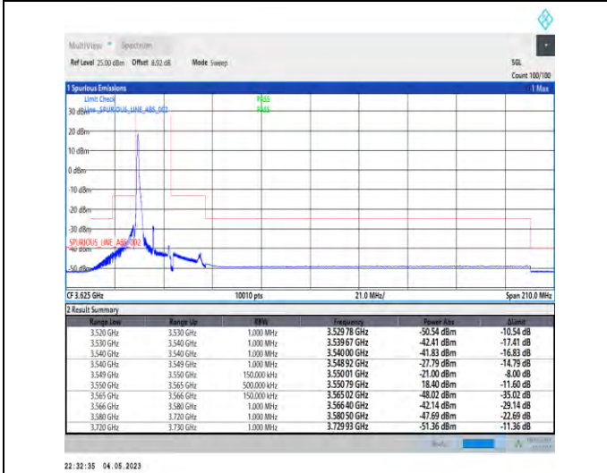
1-N48-PC3-30-15-L-4-CP-QPSK-Edge_1RB_Left-1@0-Ant1-1--PASS-see graph
