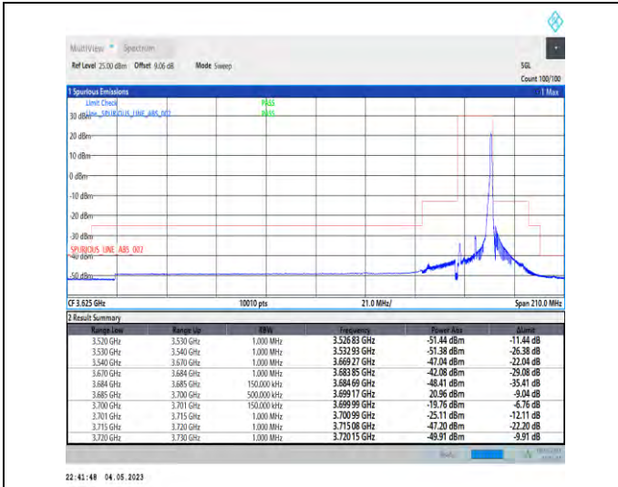
1-N48-PC3-30-15-H-2-DFT-PI2BPSK-Edge_1RB_Right-t1@37-Ant1-1--PASS-see graph
