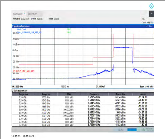
1-N48-PC3-30-30-H-3-DFT-PI2BPSK-Outer_Full-75@0-Ant1-1--PASS-see graph
