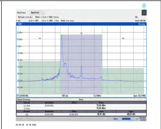
1-N48-PC3-30-40-M-CP-QPSK-Edge_1RB_Left-1@105-Ant1-1--PASS
