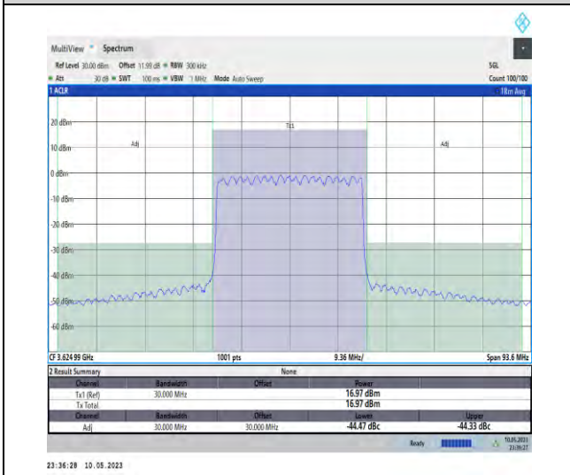
1-N48-PC3-30-30-M-CP-QPSK-Outer_Full-78@0-A nt1-1--PASS
