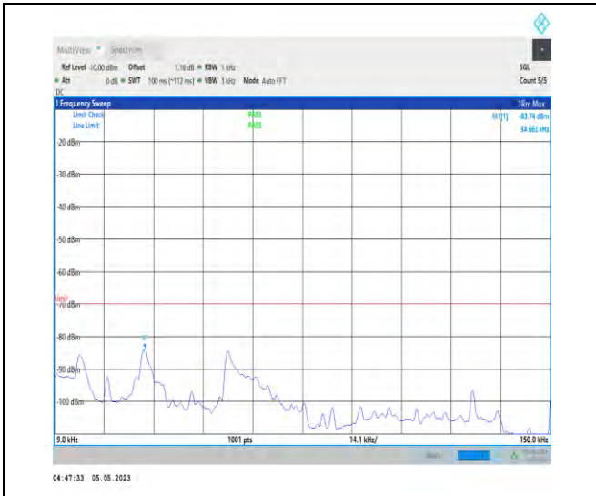
1-N48-PC3-30-40-H-1-DFT-PI2BPSK-Inner_1RB_Le ft-1@1-0.009-0.15-Ant1-0.01--112.02--70-PASS
