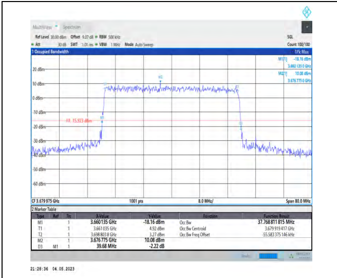
1-N48-PC3-30-40-H-7-CP-16QAM-Outer_Full-106@ 0-Ant1-37.769-39.680-≤40-PASS
