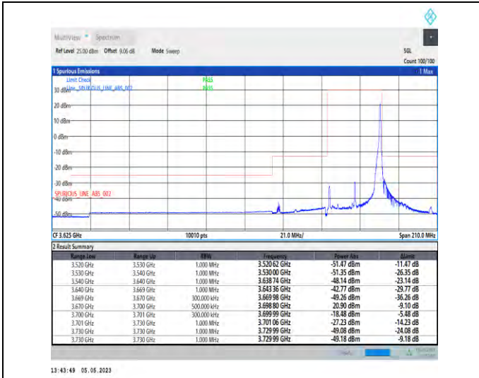
1-N48-PC3-30-30-H-2-DFT-PI2BPSK-Edge_1RB_Right-t1@77-Ant1-1--PASS-see graph
