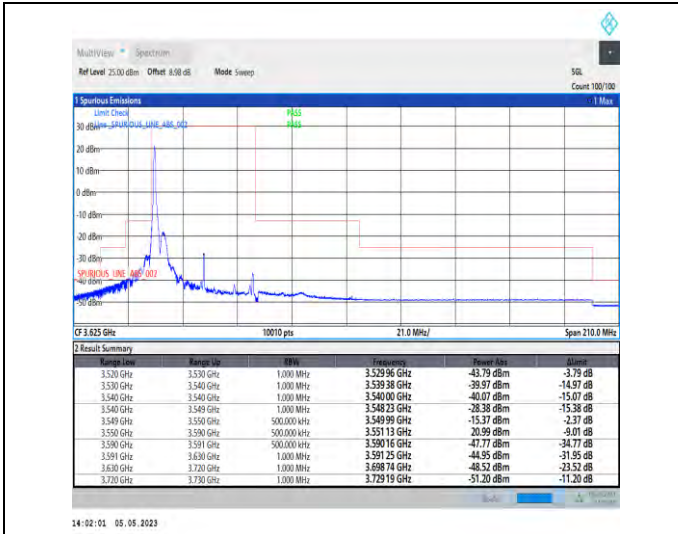
1-N48-PC3-30-40-L-1-DFT-PI2BPSK-Edge_1RB_Left-1@0-Ant1-1--PASS-see graph
