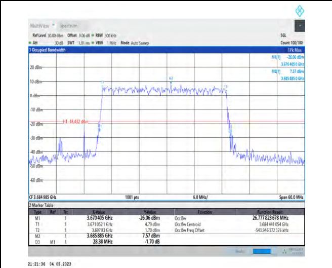
1-N48-PC3-30-30-H-5-DFT-256QAM-Outer_Full-75 @0-Ant1-26.778-28.380-<30-PASS
