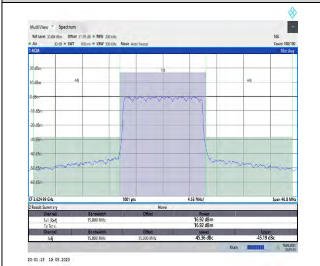
1-N48-PC3-30-15-M-CP-QPSK-Outer_Full-36@0-A nt1-1--PASS
