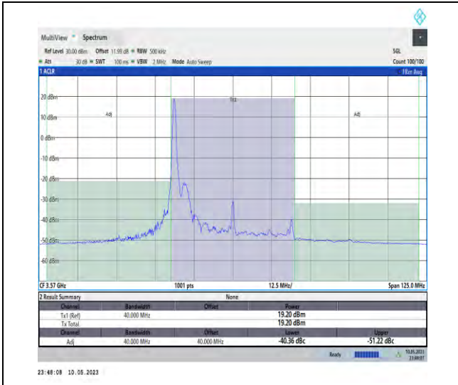
1-N48-PC3-30-40-L-DFT-PI2BPSK-Edge_1RB_Left -1@0-Ant1-1--PASS
