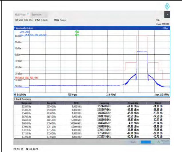
1-N48-PC3-30-15-H-6-CP-QPSK-Outer_Full-38@0-Ant1-1--PASS-see graph
