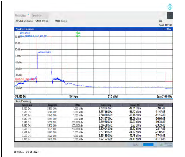
1-N48-PC3-30-20-L-3-DFT-PI2BPSK-Outer_Full-50@0-Ant1-1--PASS-see graph
