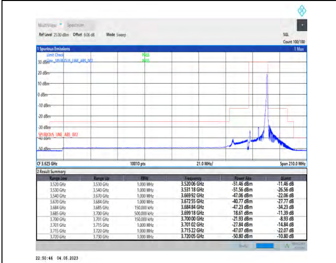
1-N48-PC3-30-15-H-5-CP-QPSK-Edge_1RB_Right1@37-Ant1-1--PASS-see graph
