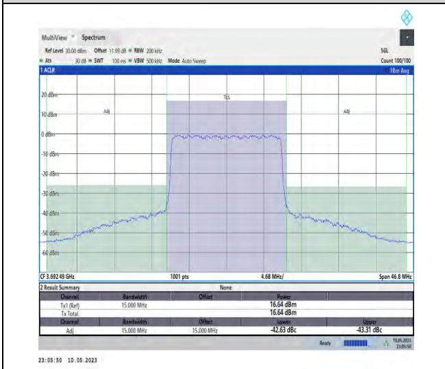
1-N48-PC3-30-15-H-CP-QPSK-Outer_Full-36@0-Ant1-1--PASS
