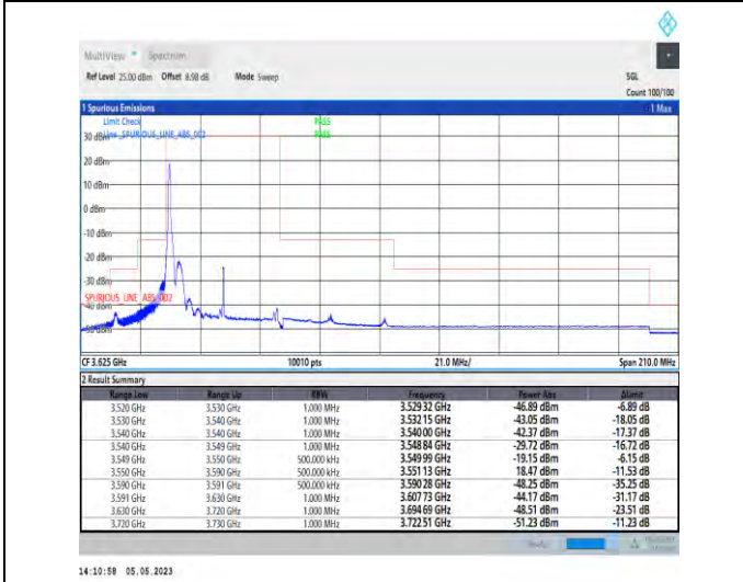
1-N48-PC3-30-40-L-4-CP-QPSK-Edge_1RB_Left-1@0-Ant1-1--PASS-see graph
