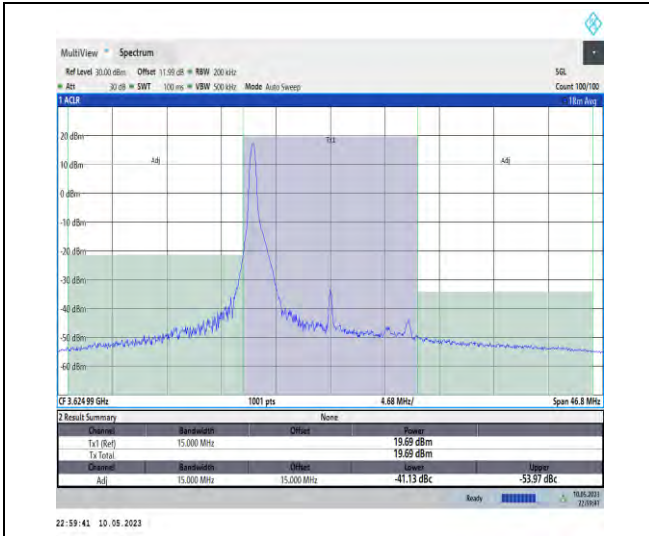
1-N48-PC3-30-15-M-DFT-PI2BPSK-Edge_1RB_Left-1@0-Ant1-1--PASS
