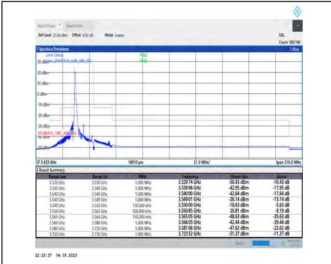
1-N48-PC3-30-15-L-1-DFT-PI2BPSK-Edge_1RB_Left-1@0-Ant1-1--PASS-see graph
