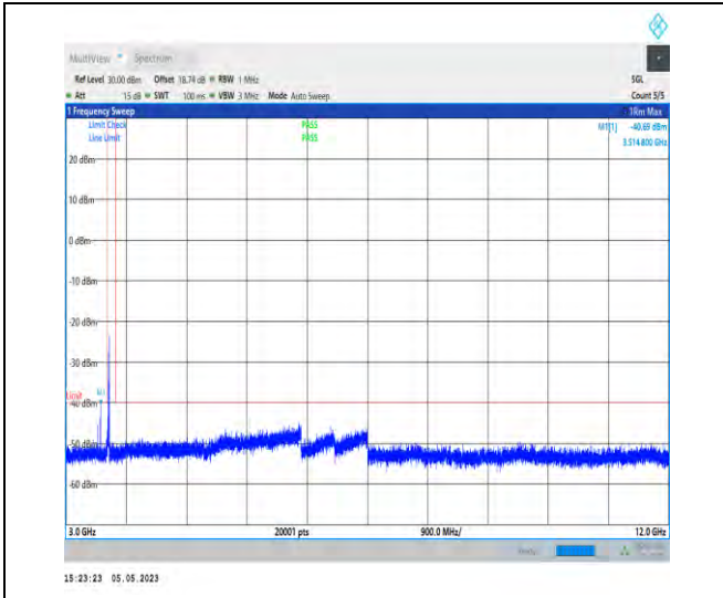
1-N48-PC3-30-40-H-1-DFT-PI2BPSK-Inner_1RB_Le ft-1@1-3000-12000-Ant1-3601.65--40.69--40-PASS
