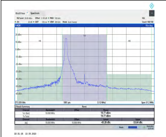
1-N48-PC3-30-10-L-DFT-PI2BPSK-Edge_1RB_Left-1@0-Ant1-1--PASS
