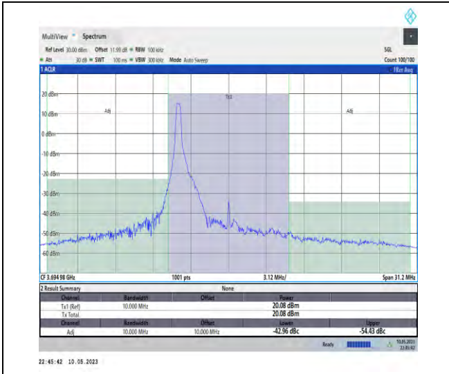
1-N48-PC3-30-10-H-DFT-PI2BPSK-Edge_1RB_Left -1@0-Ant1-1--PASS
