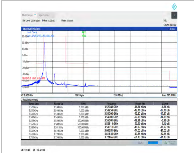
1-N48-PC3-30-30-L-1-DFT-PI2BPSK-Edge_1RB_Left-1@0-Ant1-1--PASS-see graph
