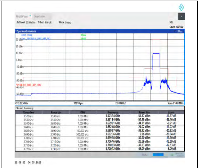
1-N48-PC3-30-10-H-3-DFT-PI2BPSK-Outer_Full-24@0-Ant1-1--PASS-see graph
