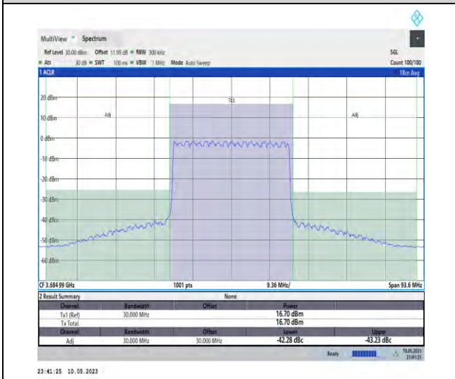
1-N48-PC3-30-30-H-CP-QPSK-Outer_Full-78@0-A nt1-1--PASS
