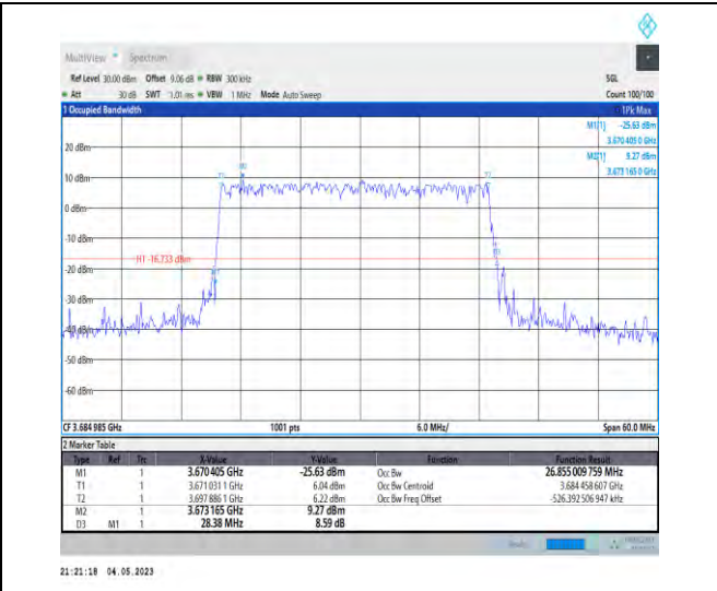
1-N48-PC3-30-30-H-3-DFT-16QAM-Outer_Full-75@ 0-Ant1-26.855-28.380-<30-PASS
