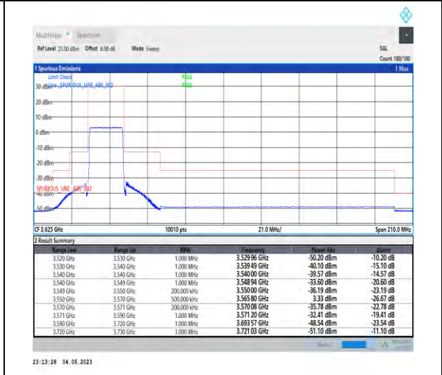
1-N48-PC3-30-20-L-6-CP-QPSK-Outer_Full-51@0-Ant1-1--PASS-see graph
