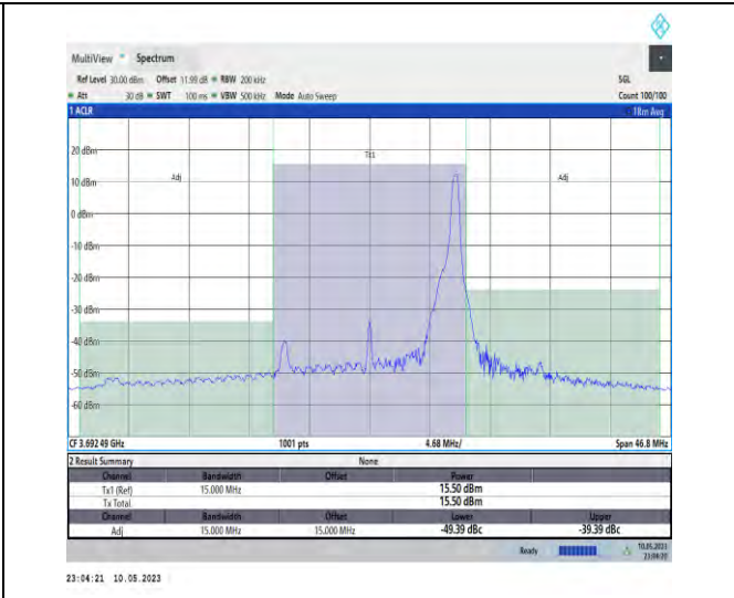
1-N48-PC3-30-15-H-CP-QPSK-Edge_1RB_Left-1@3 7-Ant1-1--PASS
