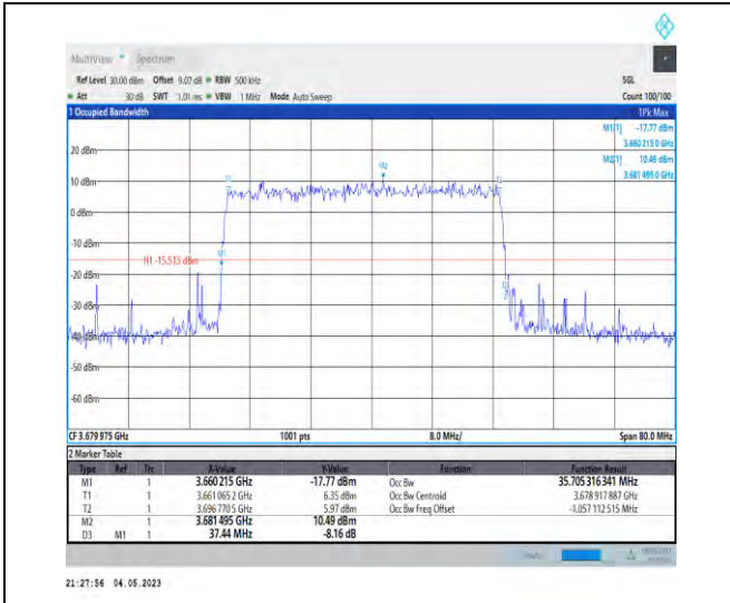
1-N48-PC3-30-40-H-3-DFT-16QAM-Outer_Full-100 @0-Ant1-35.705-37.440-≤40-PASS
