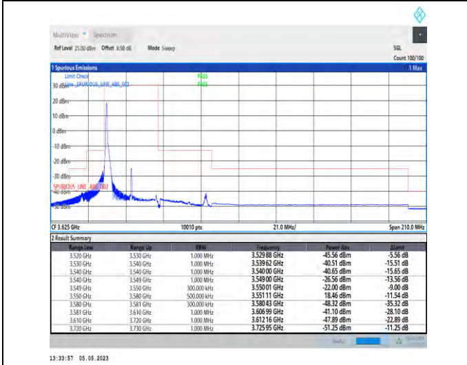
1-N48-PC3-30-30-L-4-CP-QPSK-Edge_1RB_Left-1@0-Ant1-1--PASS-see graph
