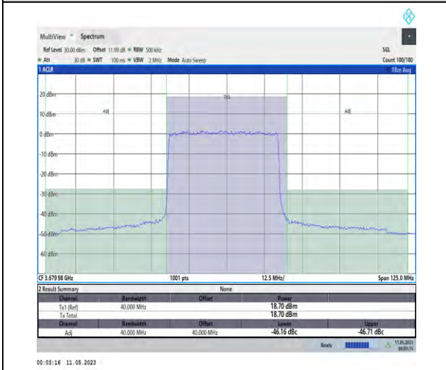
1-N48-PC3-30-40-H-DFT-PI2BPSK-Outer_Full-100@0-Ant1-1--PASS
