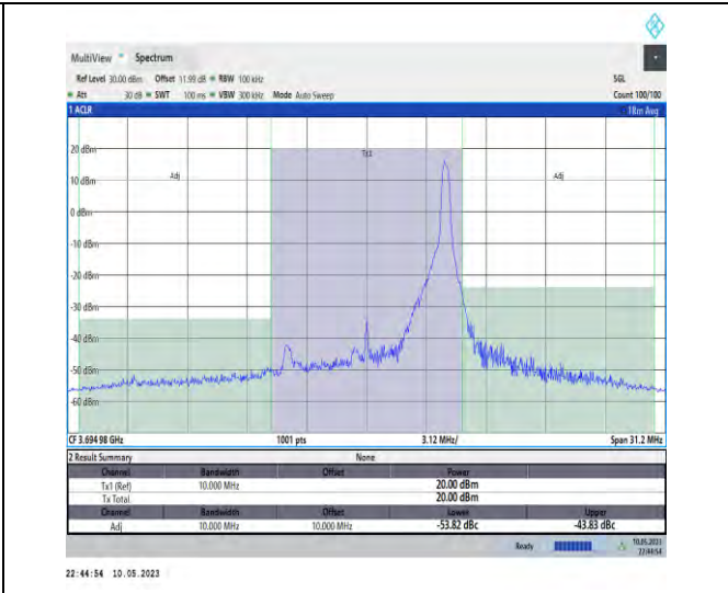
1-N48-PC3-30-10-H-DFT-PI2BPSK-Edge_1RB_Left- 1@23-Ant1-1--PASS
