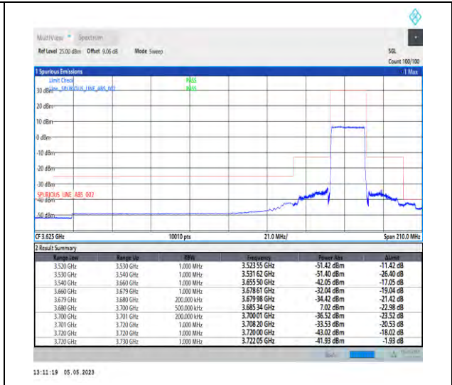
1-N48-PC3-30-20-H-3-DFT-PI2BPSK-Outer_Full-50@0-Ant1-1--PASS-see graph
