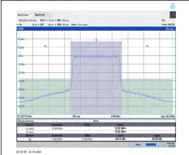
1-N48-PC3-30-15-L-CP-QPSK-Outer_Full-36@0-Ant1-1--PASS
