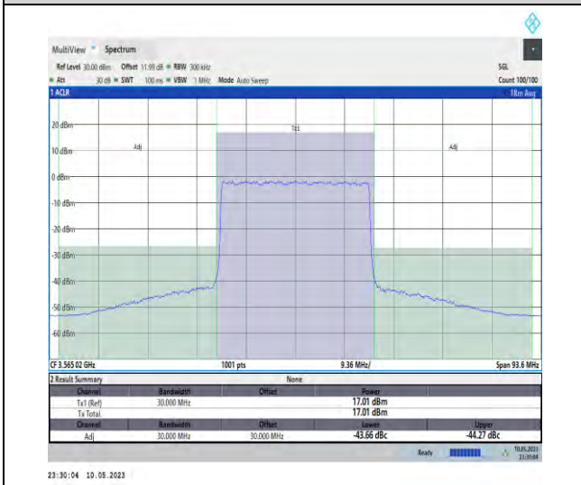
1-N48-PC3-30-30-L-CP-QPSK-Outer_Full-78@0-A nt1-1--PASS
