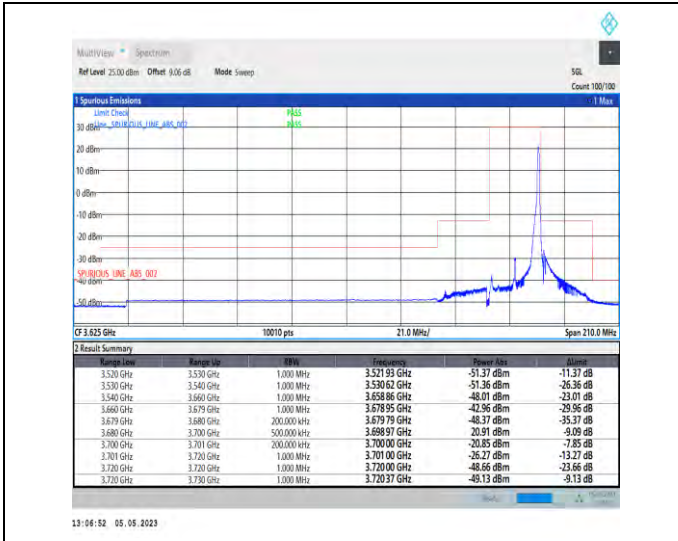
1-N48-PC3-30-20-H-2-DFT-PI2BPSK-Edge_1RB_Right-t-1@50-Ant1-1--PASS-see graph
