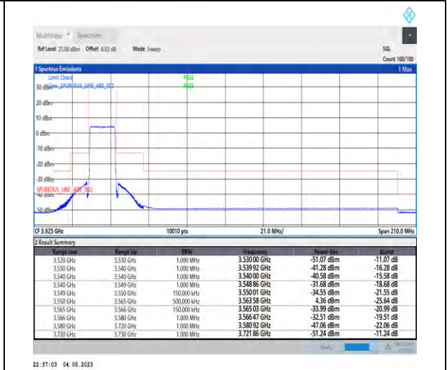
1-N48-PC3-30-15-L-6-CP-QPSK-Outer_Full-38@0-Ant1-1--PASS-see graph
