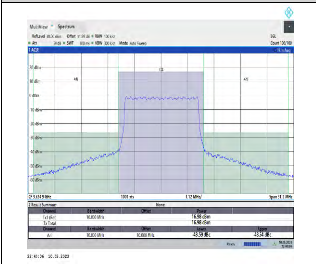
1-N48-PC3-30-10-M-CP-QPSK-Outer_Full-24@0-A nt1-1--PASS
