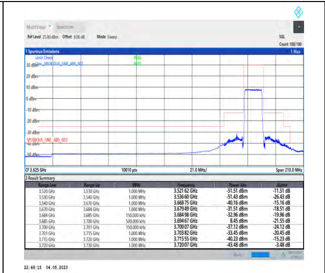
1-N48-PC3-30-15-H-3-DFT-PI2BPSK-Outer_Full-36@0-Ant1-1--PASS-see graph
