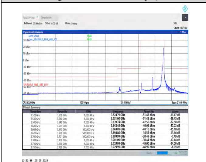
1-N48-PC3-30-30-H-5-CP-QPSK-Edge_1RB_Right-1@77-Ant1-1--PASS-see graph
