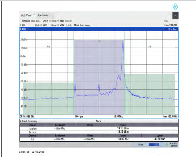
1-N48-PC3-30-40-M-DFT-PI2BPSK-Edge_1RB_Left-1@105-Ant1-1--PASS
