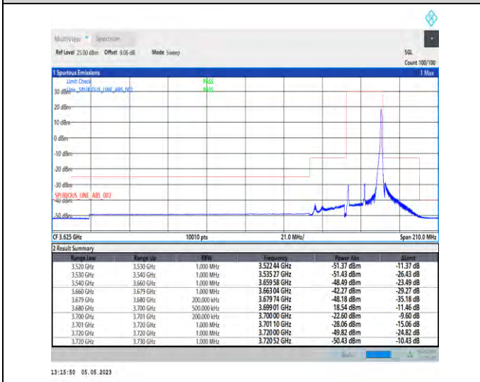
1-N48-PC3-30-20-H-5-CP-QPSK-Edge_1RB_Right-1@50-Ant1-1--PASS-see graph
