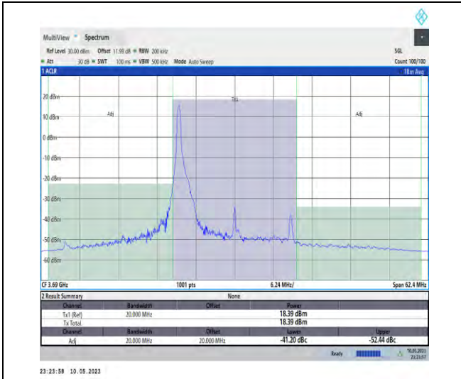
1-N48-PC3-30-20-H-DFT-PI2BPSK-Edge_1RB_Left -1@0-Ant1-1--PASS
