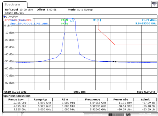
BE-NR-HIGH, SISO-B, 802.11n20-HT0, Ch169
