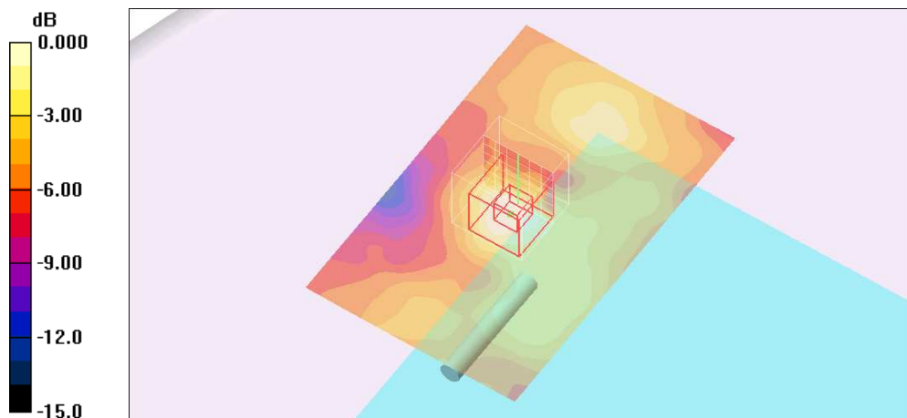
0 dB = 0.025mW/g
