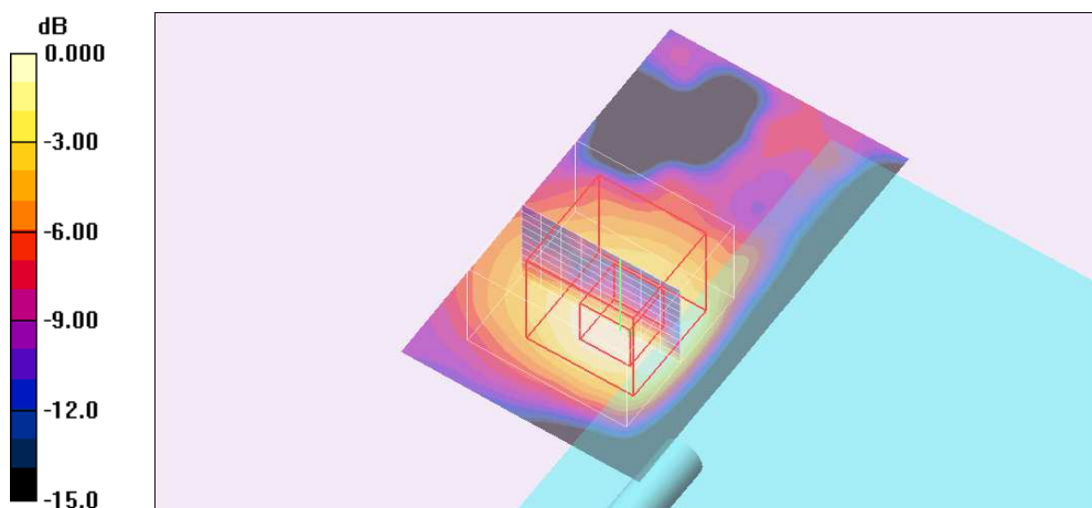
0 dB = 0.647mW/g
