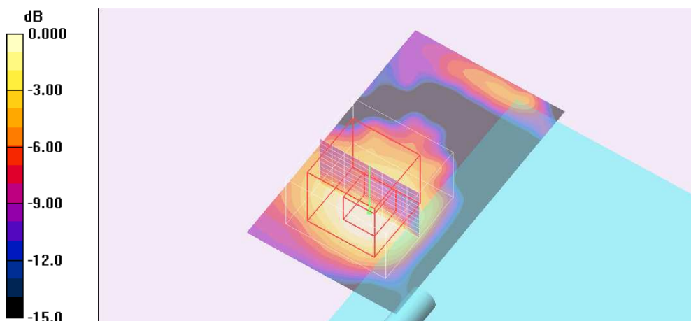
0 dB = 0.514mW/g
