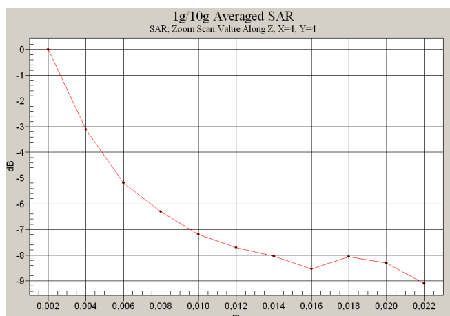
0 dB = 0.514mW/g
