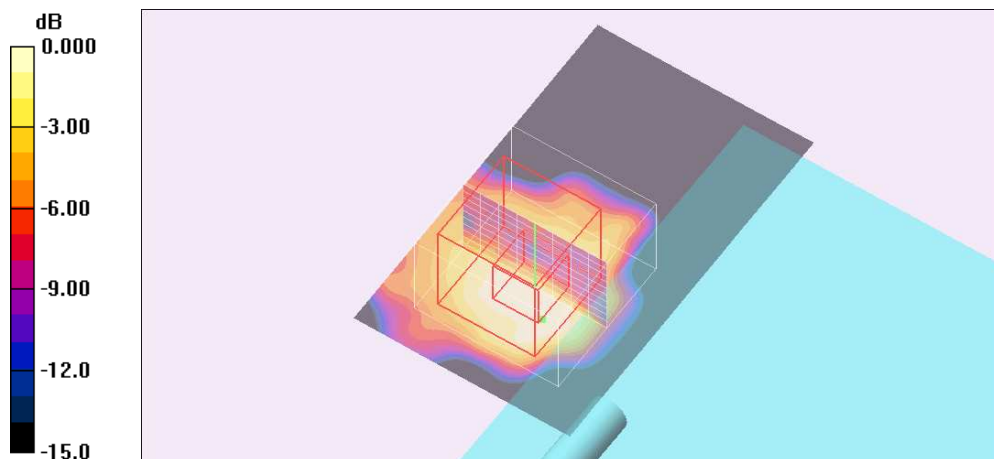
0 dB = 0.440mW/g
