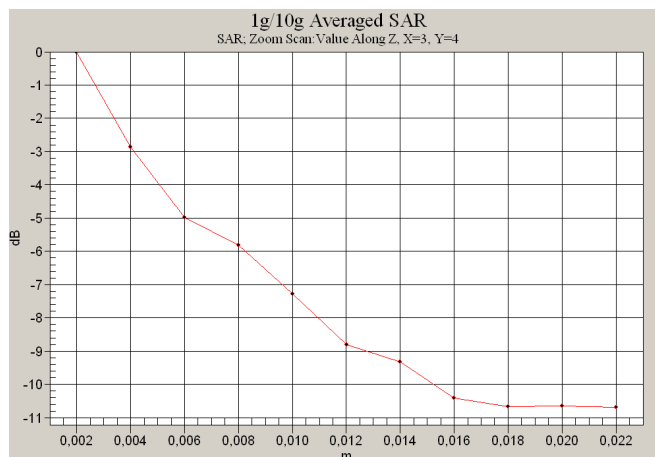
0 dB = 0.647mW/g
