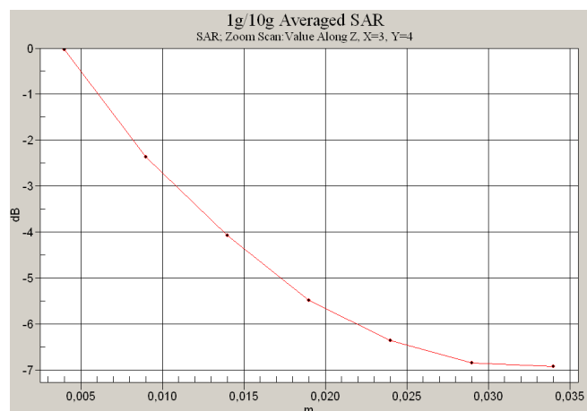
0 dB = 0.025mW/g
