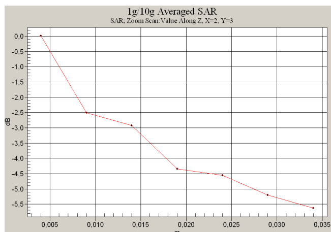
0 dB = 0.022mW/g
