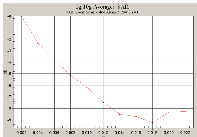
0 dB = 0.342mW/g
