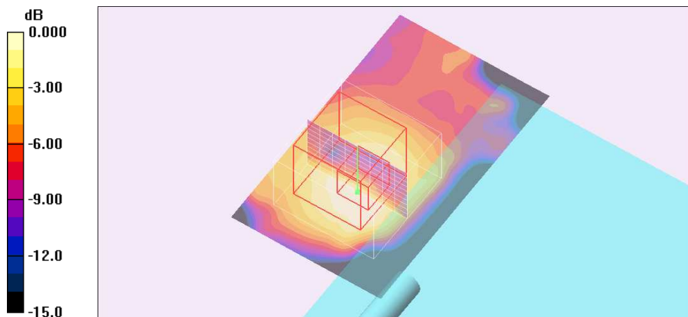
0 dB = 0.342mW/g
