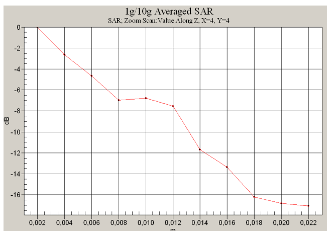
0 dB = 0.666mW/g
