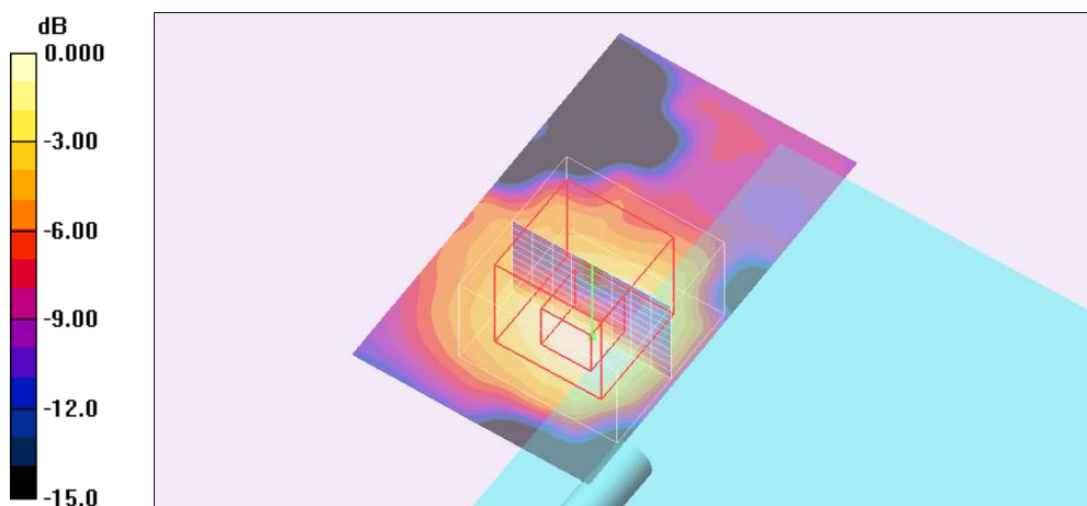
0 dB = 0.666mW/g
