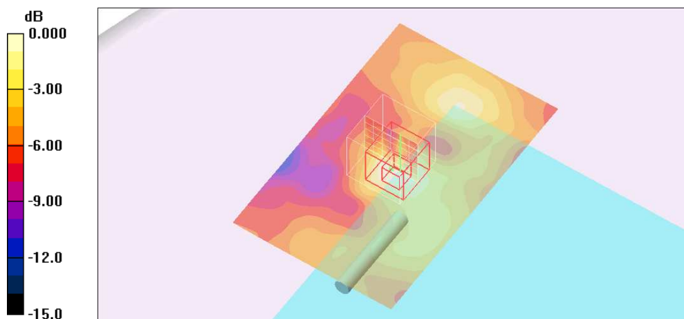
0 dB = 0.022mW/g
