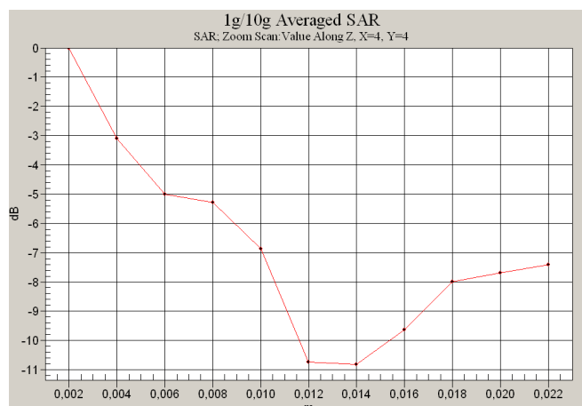
0 dB = 0.440mW/g
