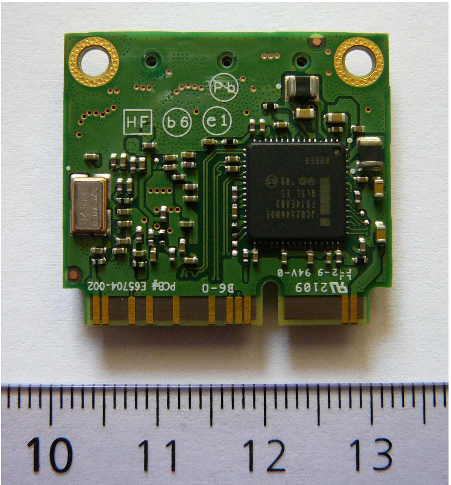
Bottom View
