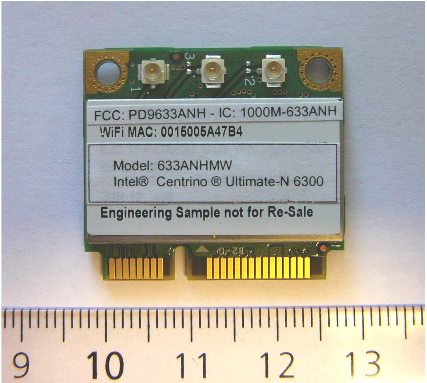
Top View
