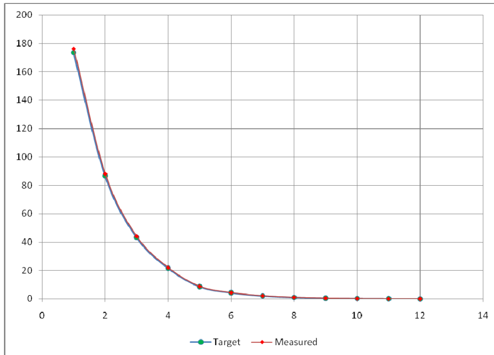
Probe Linearity @ 2600MHz CW
