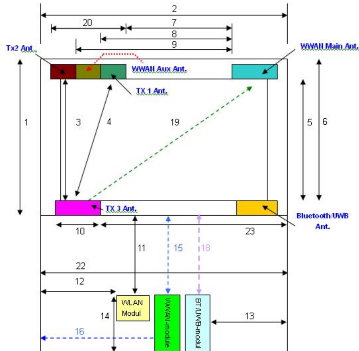
Antenna Locations
