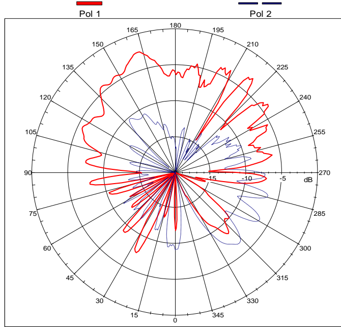
Far-Field Phi Cut, Theta=90 f=5.8500 GHz
