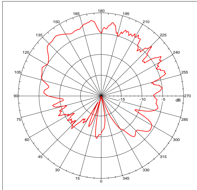
Far-Field Pwr SumPhi Cut, Theta=90 f=5.6000 GHz
