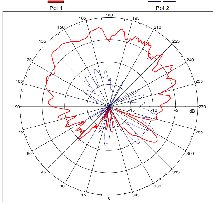
Far-Field Phi Cut, Theta=90 f=5.6000 GHz
