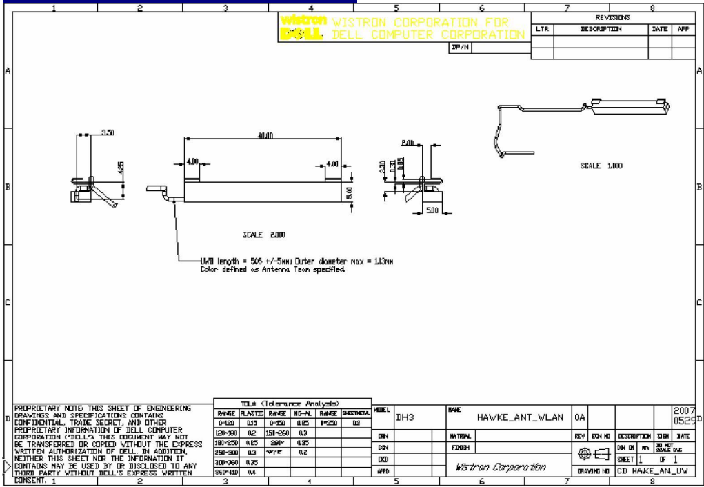
Tx1 Antenna Dimensioned Drawing:
