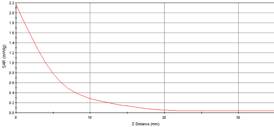
SAR - Z Axis at Hotspot x:15.0 y:-31.0
