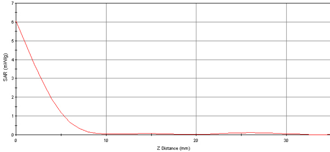
SAR - Z Axis at Hotspot x:11.0 y:-35.0
