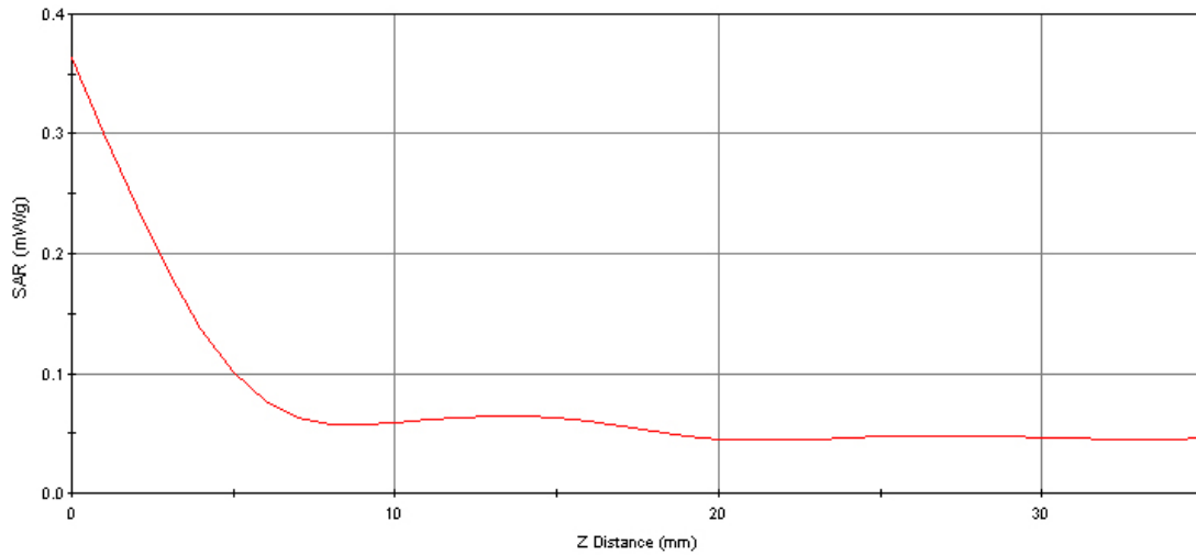
SAR - Z Axis at Hotspot x:35.0 y:52.0
