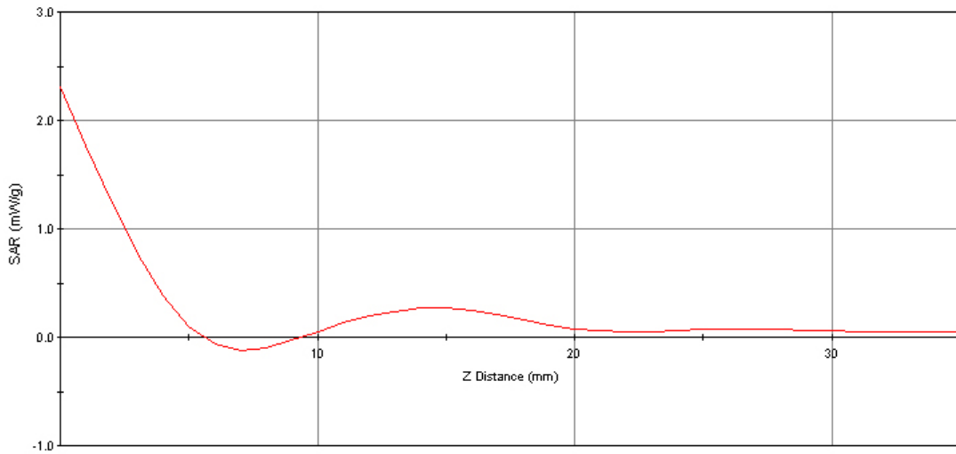
SAR - Z Axis at Hotspot x:52.0 y:46.0
