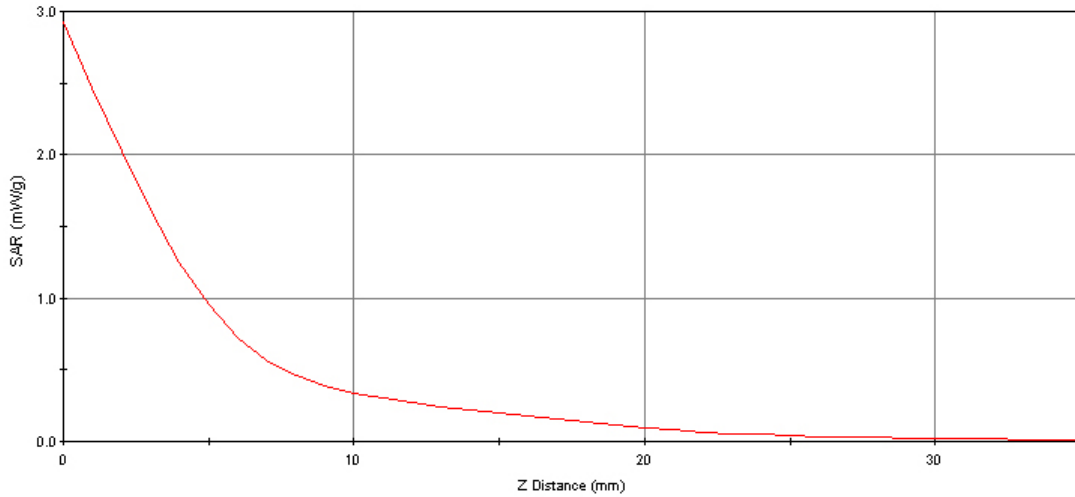
SAR - Z Axis at Hotspot x:15.0 y:-26.0
