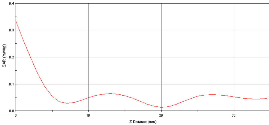
SAR - Z Axis at Hotspot x:23.0 y:68.0
