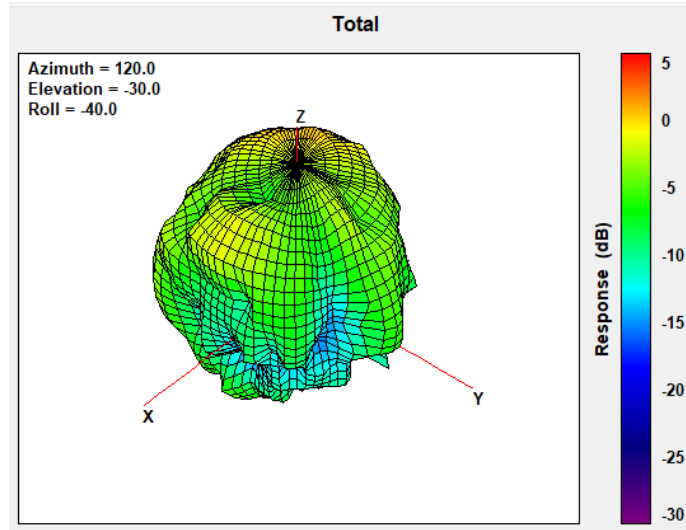
Max Antenna 3D Radiation Pattern 5250-5350 MHz
