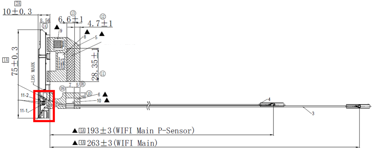
Main Antenna Drawing:
