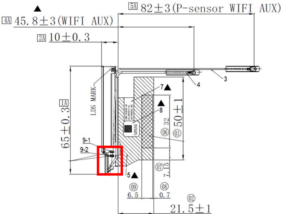
Aux Antenna Drawing:
