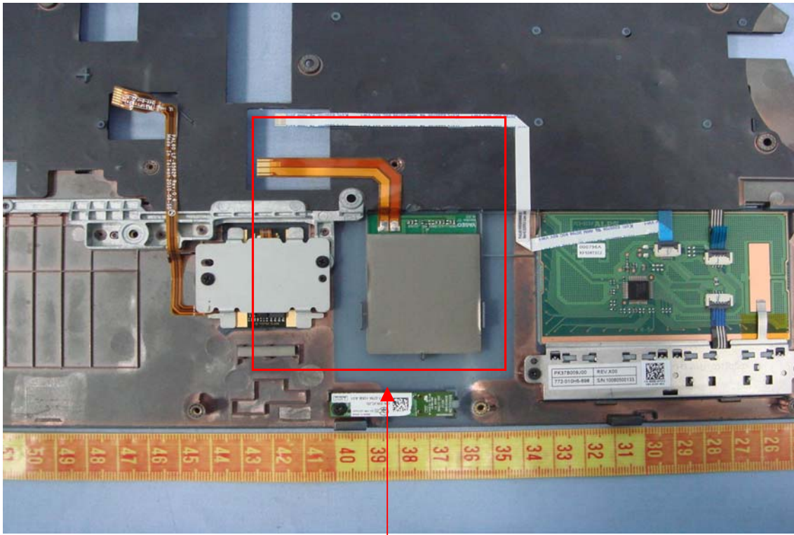
Antenna Location
