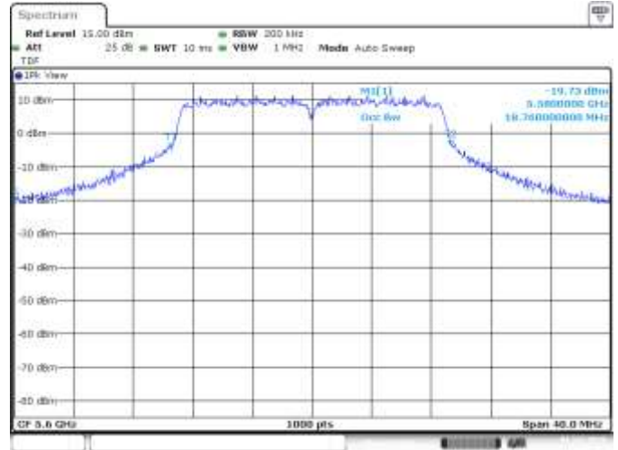
SISO A, CH120, 802.11n20, HT0, 99%
