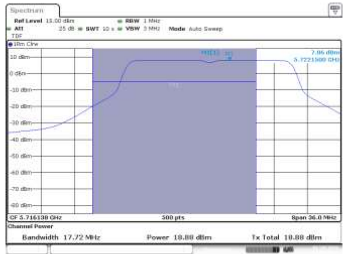
MIMO B, 802.11n20, Overlapped CH144
