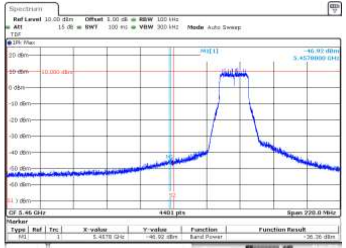
MIMO A, 802.11ax20, HE0, CH100, BE Low Peak (Restricted)
