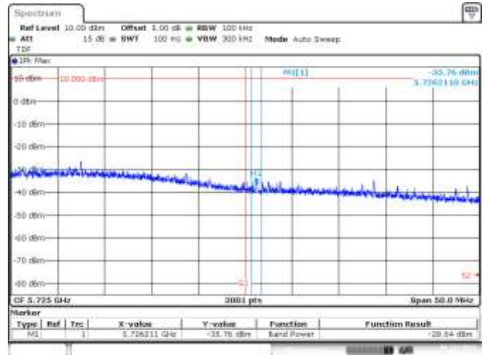
SISO B, 802.11ax40, HE0, CH134, BE High Peak
