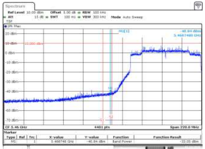
MIMO A, 802.11ax80, HE0, CH106, BE Low Peak (Restricted)
