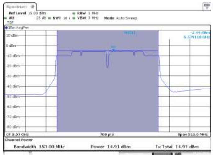
SISO A, CH114, 802.11ac160, VHT0
