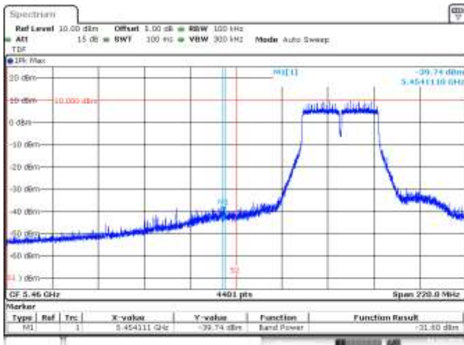
SISO A, 802.11n40, HT0, CH102, BE Low Peak (Restricted)
