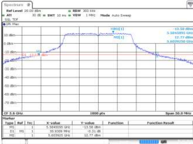
SISO A, CH120, 802.11n20, HT0, 26dB
