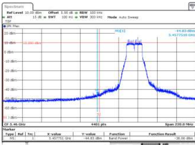
SISO B, 802.11n20, HT0, CH100, BE Low Peak (Restricted)
