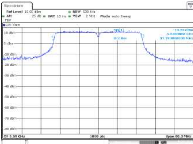
SISO A, CH118, 802.11n40, HT0, 99%
