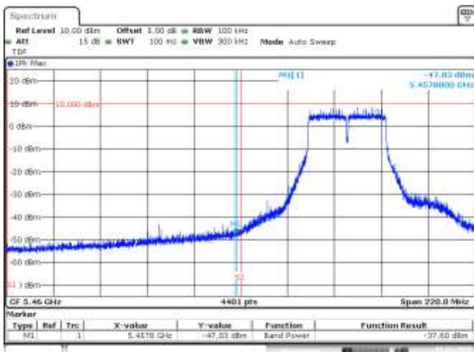
MIMO A, 802.11n40, HT8, CH102, BE Low Peak (Restricted)
