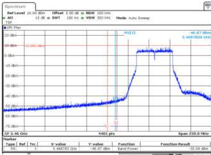
SISO B, 802.11ax40, HE0, CH102, BE Low Peak (Restricted)
