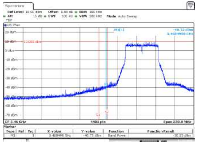
SISO A, 802.11ax40, HE0, CH102, BE Low Peak (Restricted)
