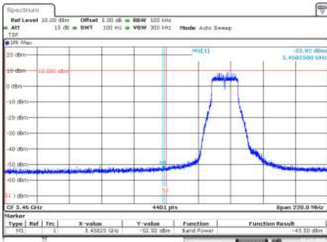
MIMO B, 802.11n20, HT8, CH100, BE Low Peak (Restricted)
