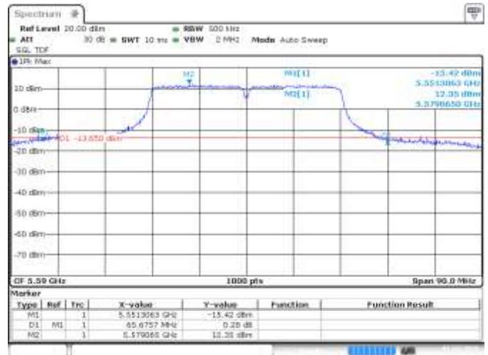
SISO A, CH118, 802.11n40, HT0, 26dB
