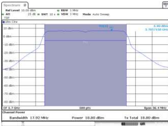
SISO A, CH140, 802.11n20, HT0
