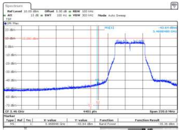
MIMO A, 802.11ax40, HE0, CH102, BE Low Peak (Restricted)
