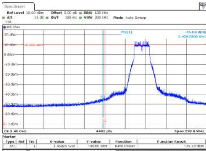
SISO B, 802.11a, 6Mbps, CH100, BE Low Peak (Restricted)
