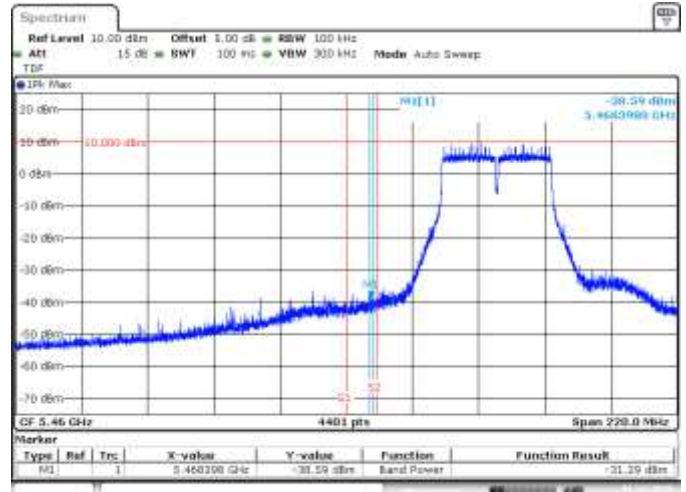
SISO A, 802.11n40, HT0, CH102, BE Low Peak (Non Restricted)
