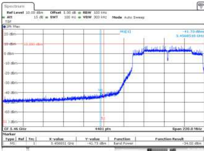
SISO B, 802.11ac80, VHT0, CH106, BE Low Peak (Restricted)
