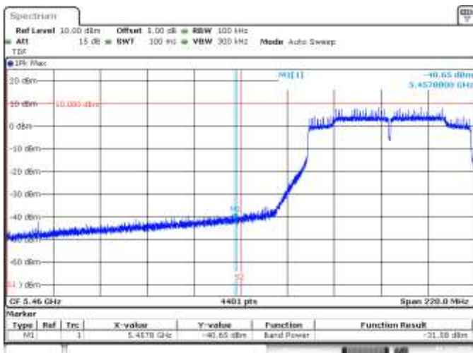
MIMO B, 802.11ac80, VHT0, CH106, BE Low Peak (Restricted)
