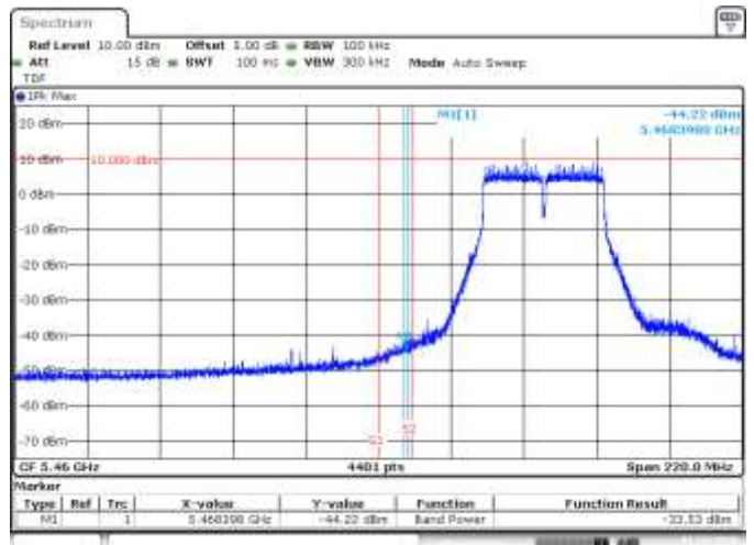
MIMO B, 802.11n20, HT8, CH100, BE Low Peak (Non Restricted)
