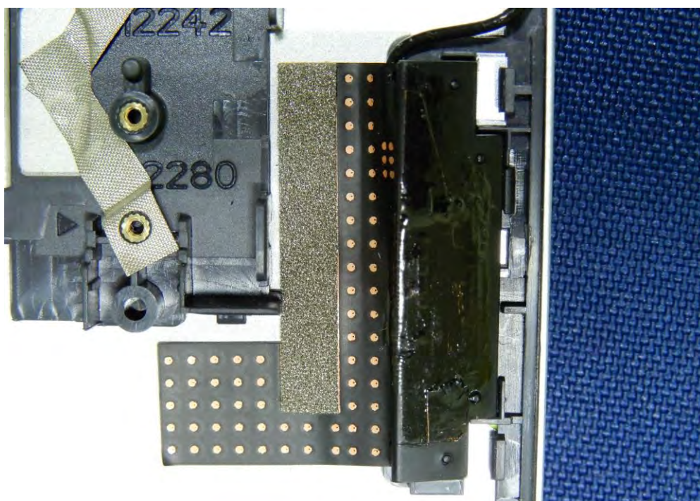
WNC Aux Antenna Part No. 025.901MP.0011
