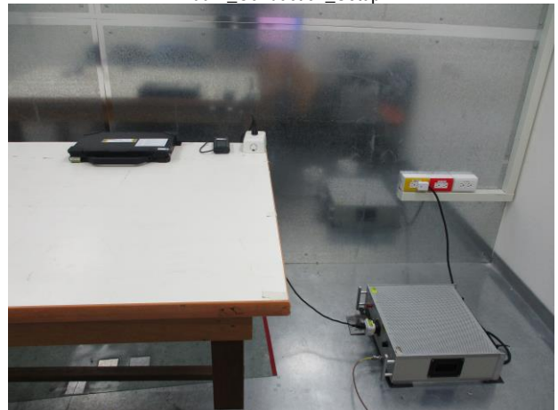
100W_Conduction_Setup
