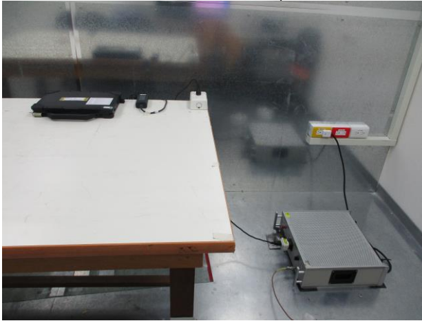
65W_Conduction_Setup
