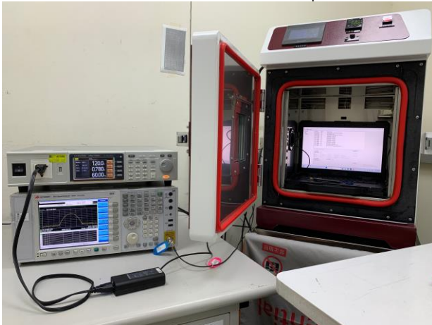
IC RSS_NFC_Conducted_Setup
