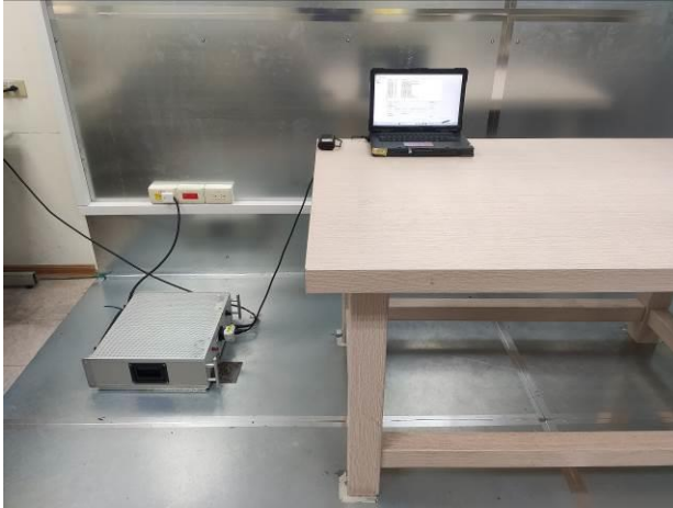
FCC_15_225+RSS_210_NFC_Conduction_100W Adapter setup photo(2)
