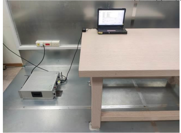
FCC_15_225+RSS_210_NFC_Conduction_65W Adapter setup photo(2)
