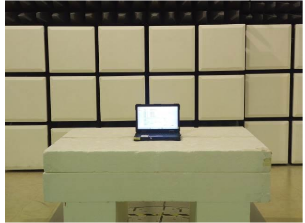
FCC_15_225+RSS_210_NFC_Radiated_Setup
