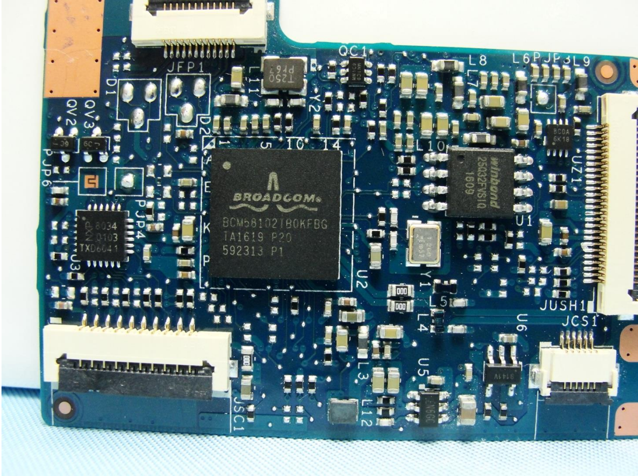
EUT: RFID 13.56MHz Wireless Module (Brand Name: DELL / Model Name: DWRFID1602)
