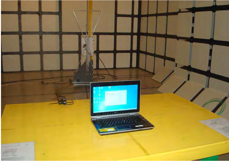
30MHz ~ 1GHz _ Rear View _ Mode 4
