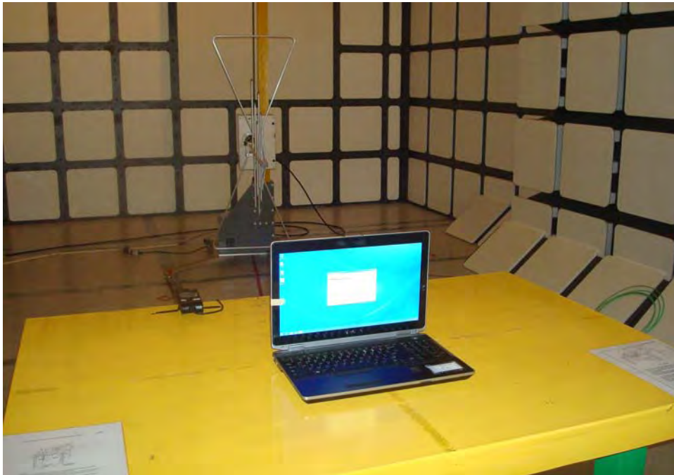
30MHz ~ 1GHz _ Rear View _ Mode 9
