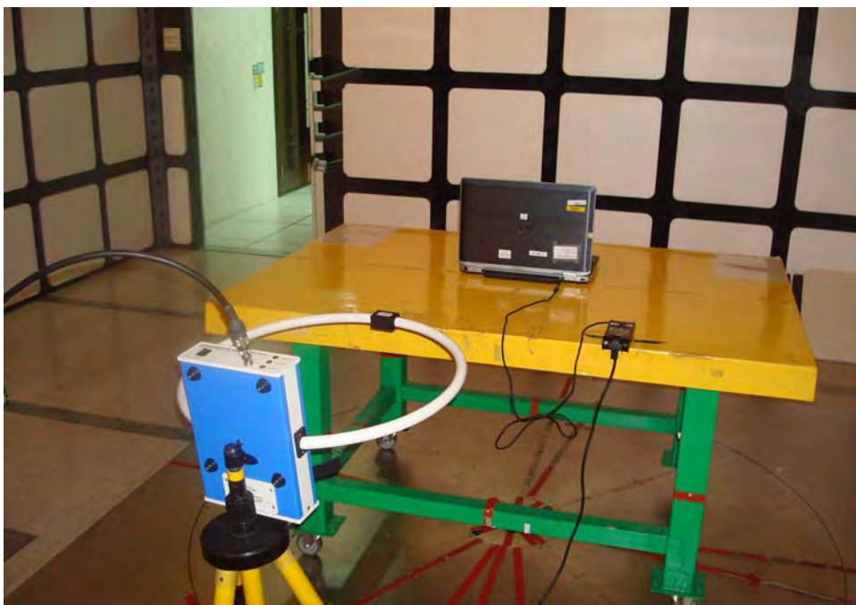
Below 30MHz _ Rear View _ Mode 9
