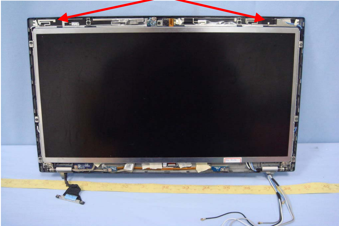
Antenna Location
