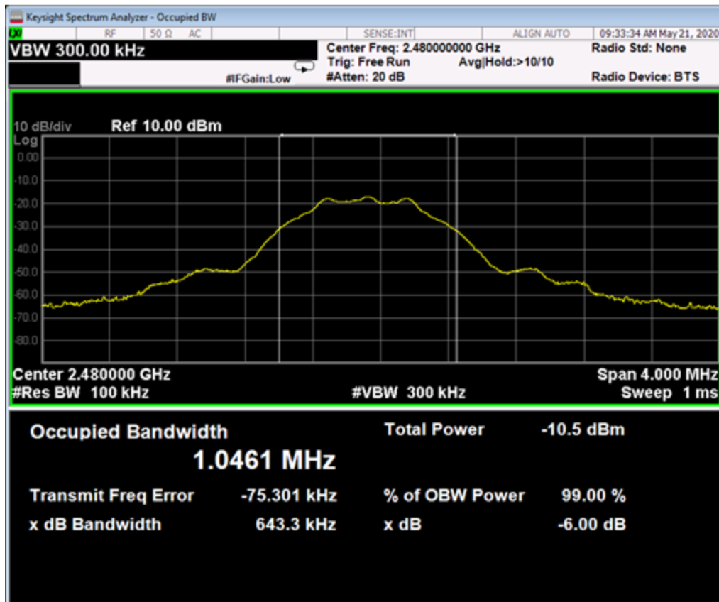
6dB Bandwidth – High Channel
