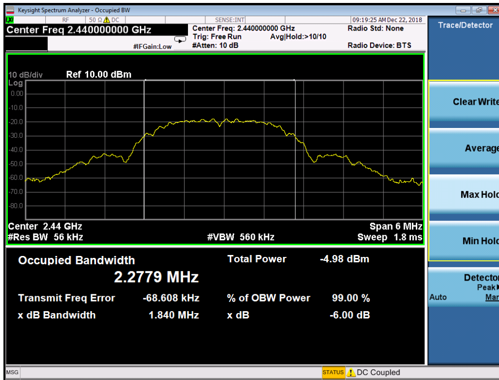
Occupied Bandwidth, Mid Channel
