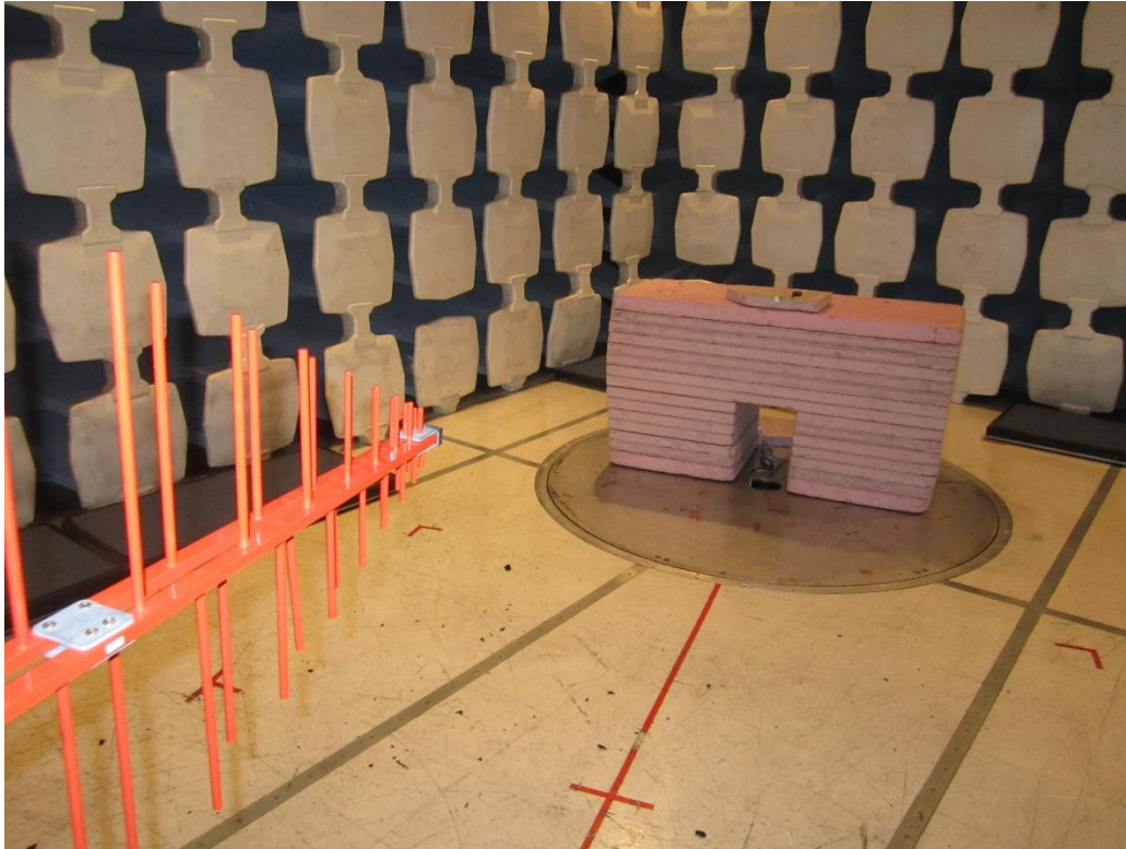
30MHz-1GHz
