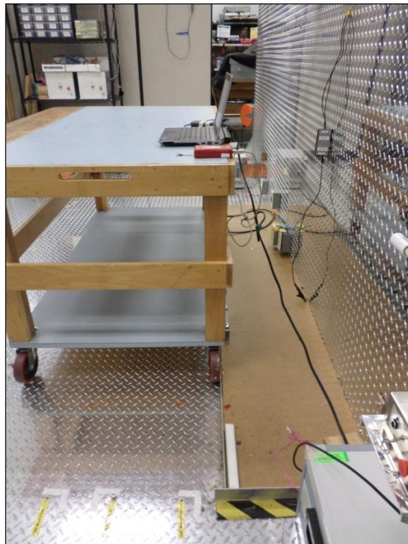
Photograph 2. Conducted Emissions, 15.207(a), Test Setup, LISN
