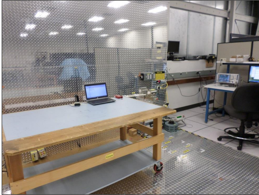
Photograph 1. Conducted Emissions, 15.207(a), Test Setup, Front
