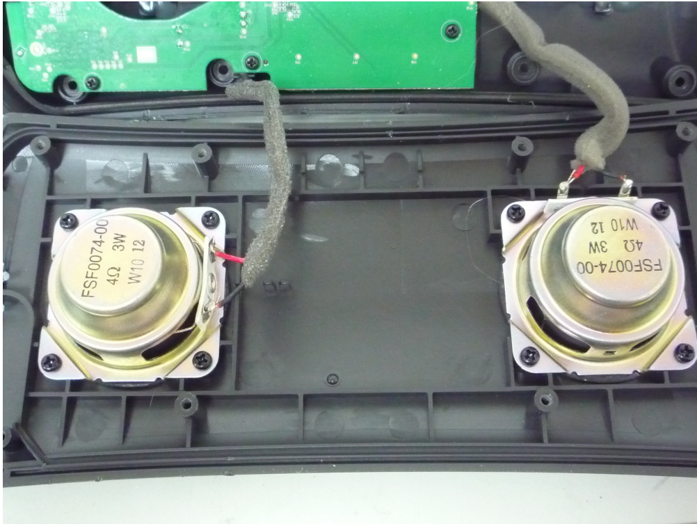
Fig. 3: Internal view
