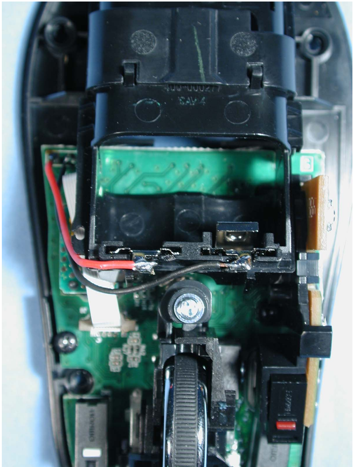
Photograph 2: M-RCH105 internal view (close-up)
